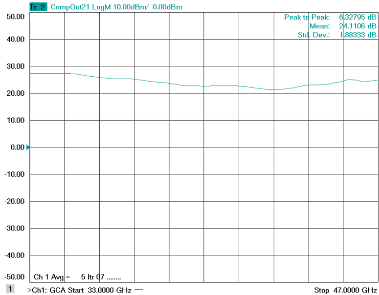
Figure 1: ERZ-HPA-3300-4700-24-E Psat
