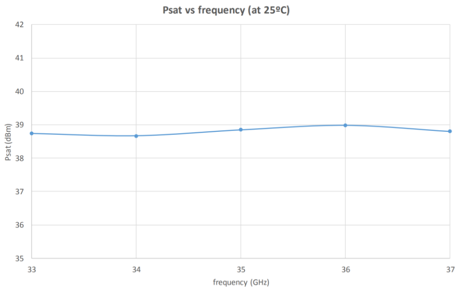
Figure 1: ERZ-HPA-3300-3700-40-W Psat
