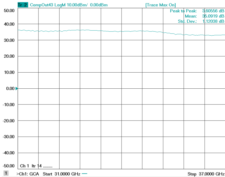
Figure 1: ERZ-HPA-3100-3700-33 Psat
