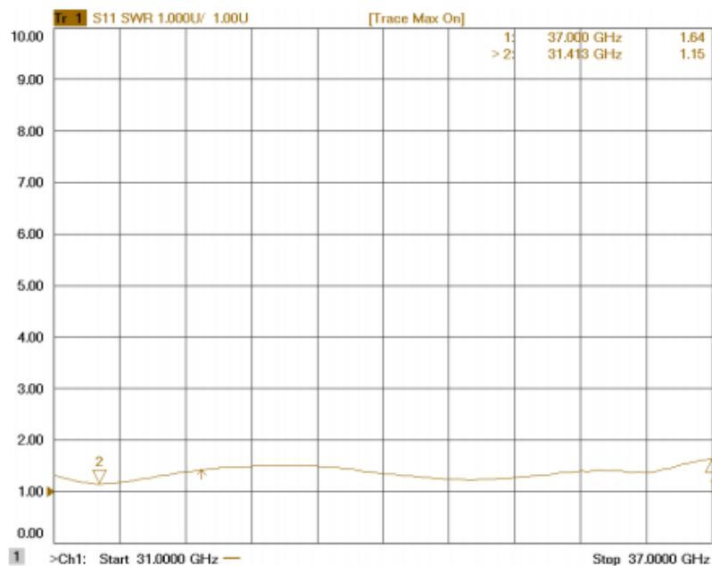
Figure 4: ERZ-HPA-3100-3700-33-W Input Matching
