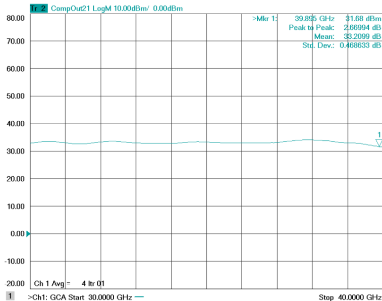
Figure 1-1: ERZ-HPA-3000-4000-32 Psat
