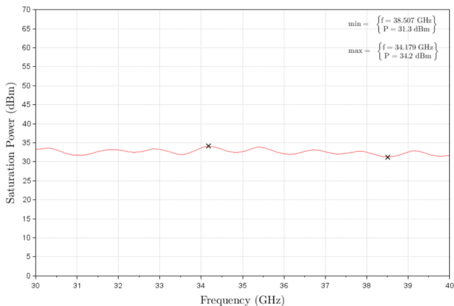
Figure 1: ERZ-HPA-3000-4000-32-E-W Psat
