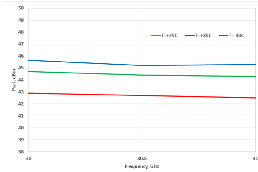
Figure 1: ERZ-HPA-3000-3100-46 Psat
