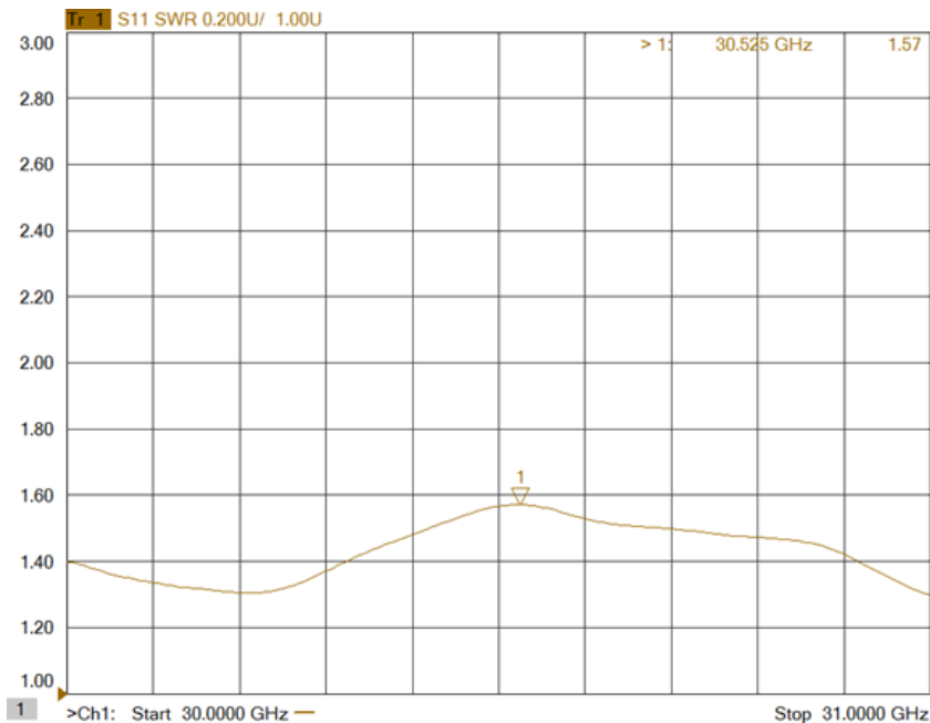
Figure 4: ERZ-HPA-3000-3100-46 Output Matching
