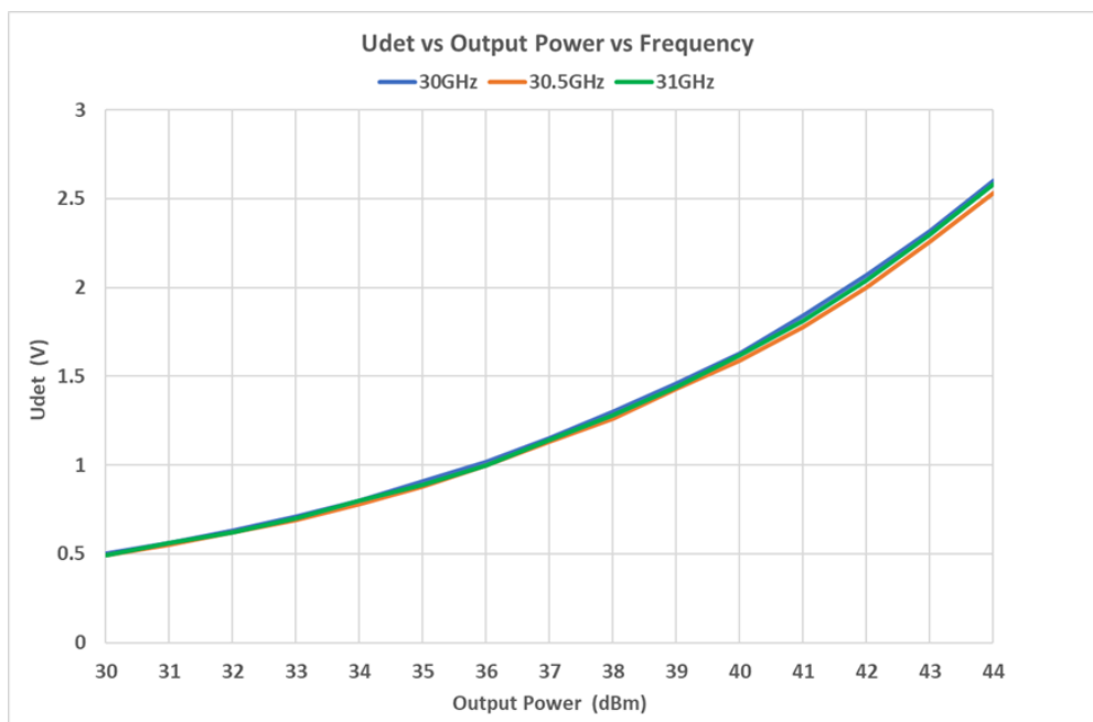
Figure 7: ERZ-HPA-3000-3100-46 Output power detector
