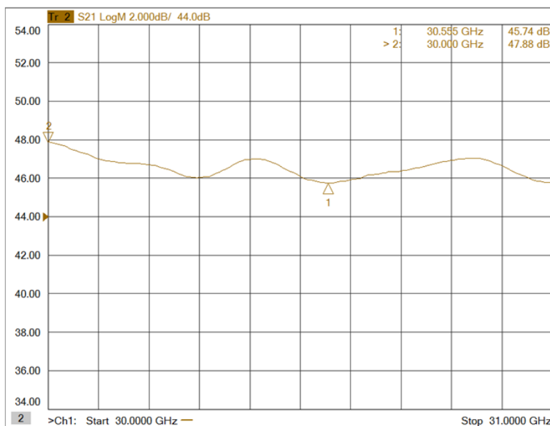
Figure 2: ERZ-HPA-3000-3100-46 Small Signal Gain
