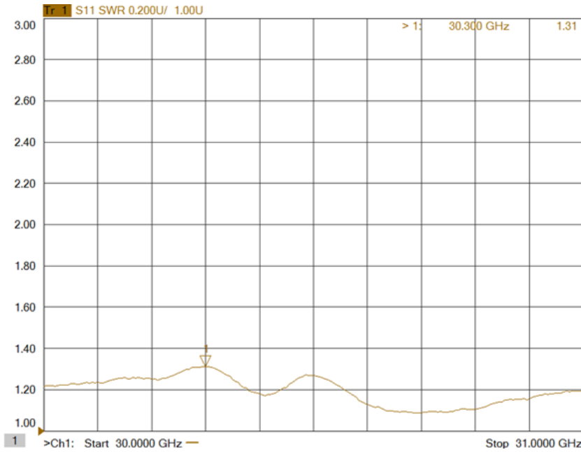
Figure 3: ERZ-HPA-3000-3100-46 Input Matching
