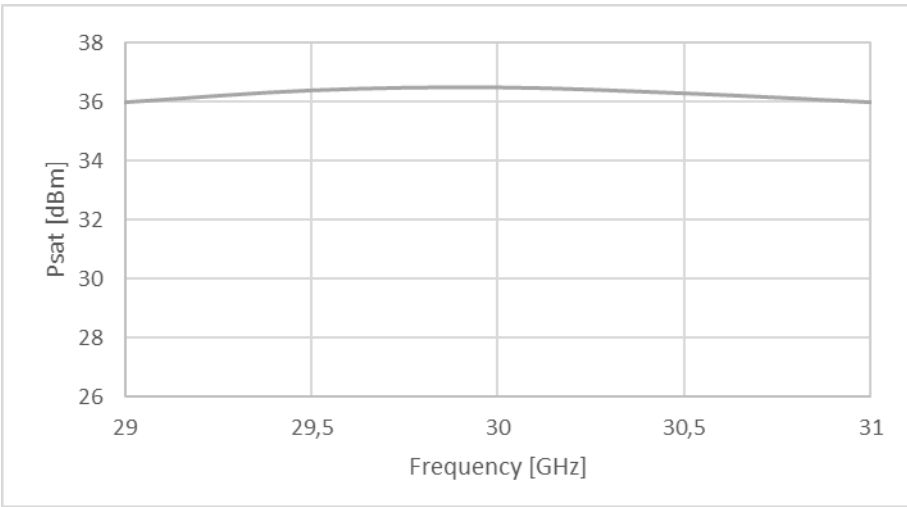
Figure 1: ERZ-HPA-2900-3100-37 Psat
