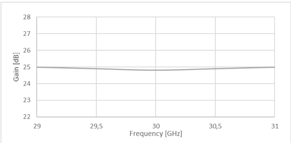
Figure 2: ERZ-HPA-2900-3100-37 Small Signal Gain
