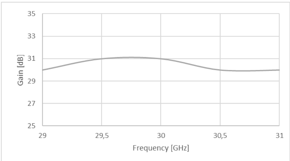
Figure 2: ERZ-HPA-2900-3100-37-E Small Signal Gain
