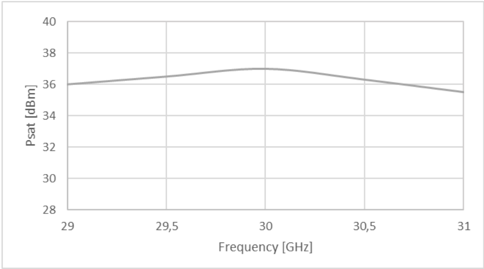
Figure 1: ERZ-HPA-2900-3100-37-E Psat
