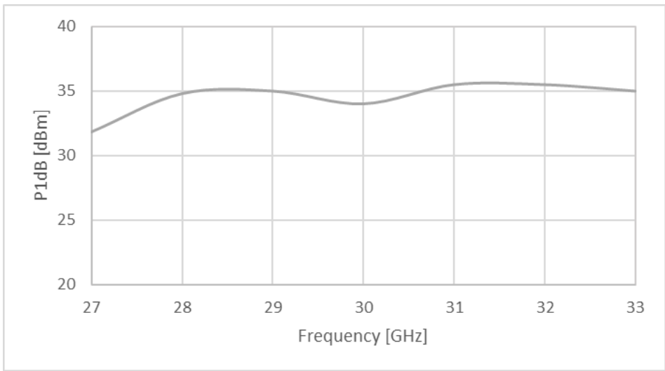
Figure 1: ERZ-HPA-2800-3300-33 P1dB
