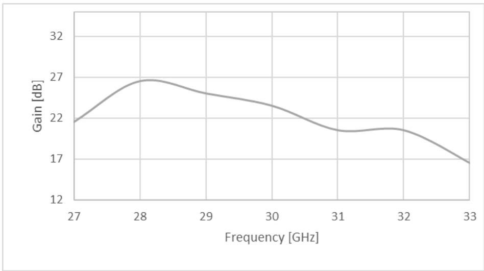
Figure 2: ERZ-HPA-2800-3300-33 Small Signal Gain
