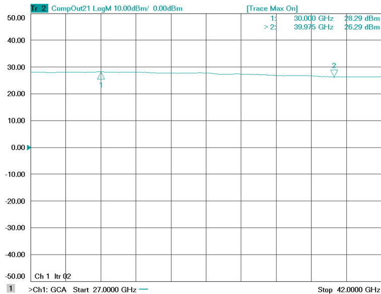
Figure 1-1: ERZ-HPA-2700-4200-27 Psat
