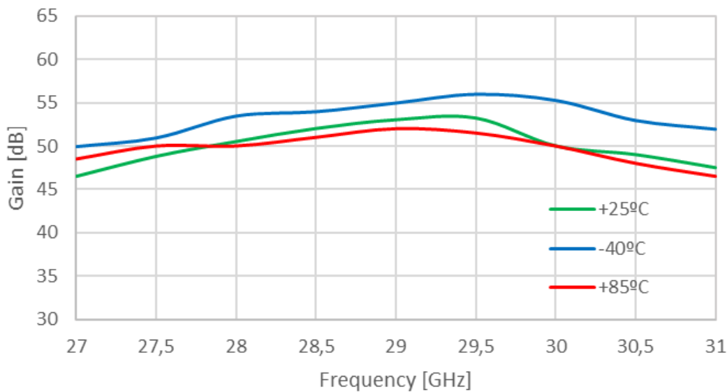
Figure 2: ERZ-HPA-2700-3100-43 Small Signal Gain
