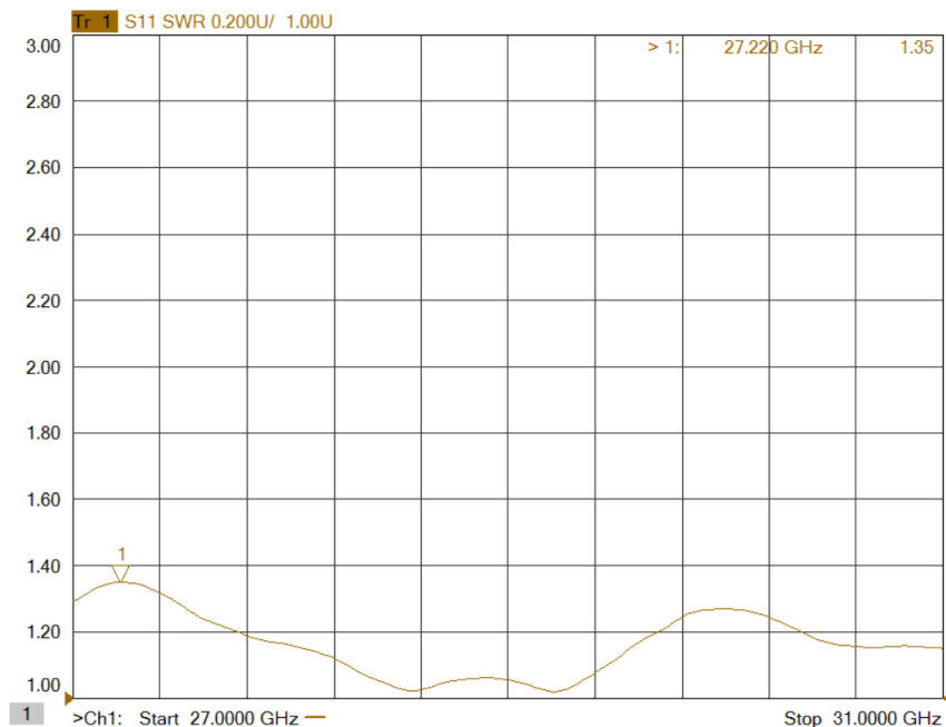
Figure 4: ERZ-HPA-2700-3100-43 Output Matching
