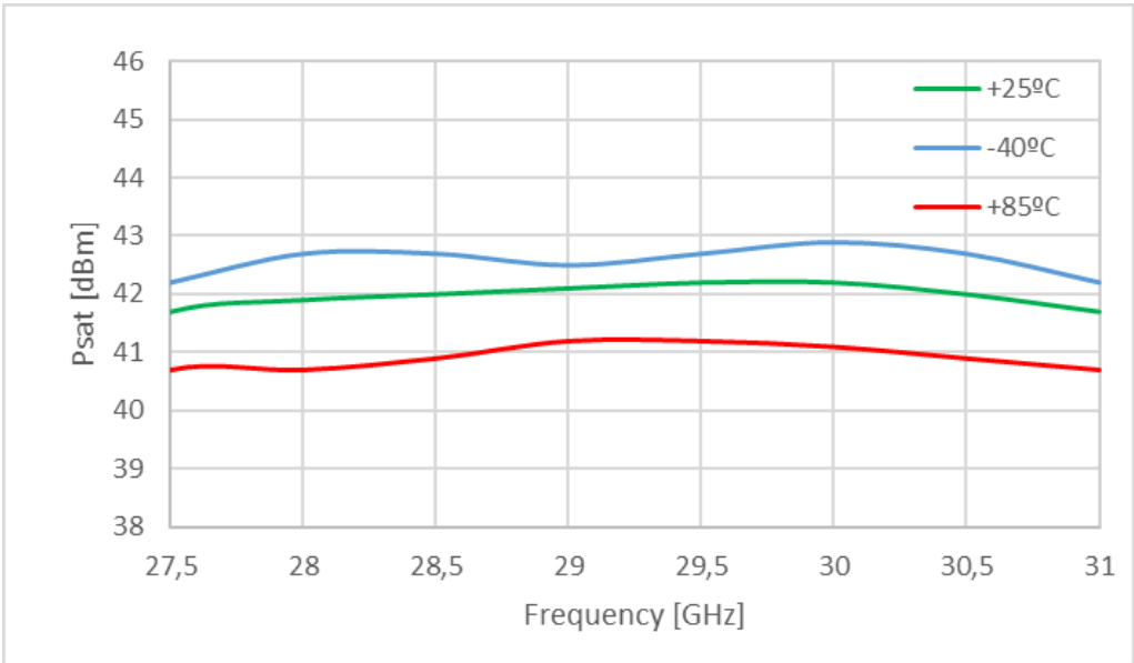
Figure 1: ERZ-HPA-2700-3100-43 Psat
