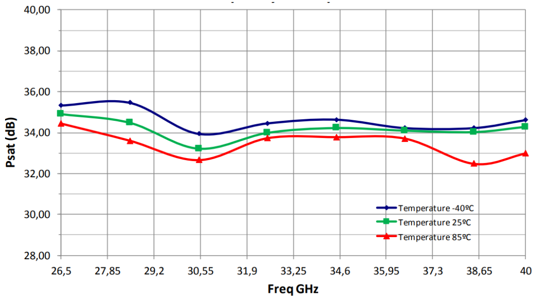
Figure 1: ERZ-HPA-2650-4000-33 Psat
