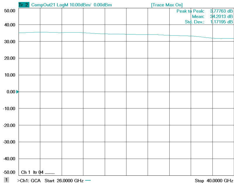
Figure 1: ERZ-HPA-2600-4000-33 Psat
