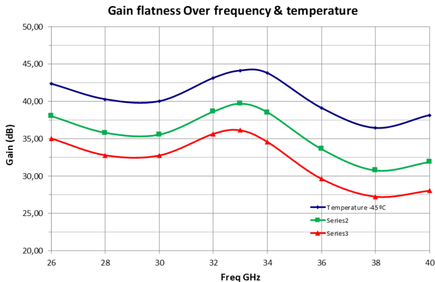
Figure 5: ERZ-HPA-2600-4000-33-A Gain flatness
