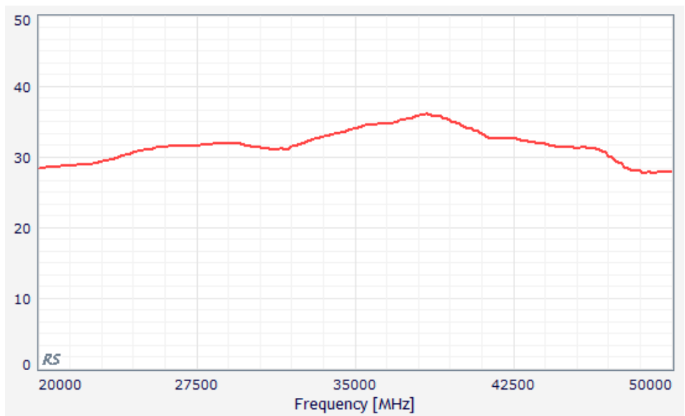
Figure 2: ERZ-HPA-2400-5000-28 Small Signal Gain
