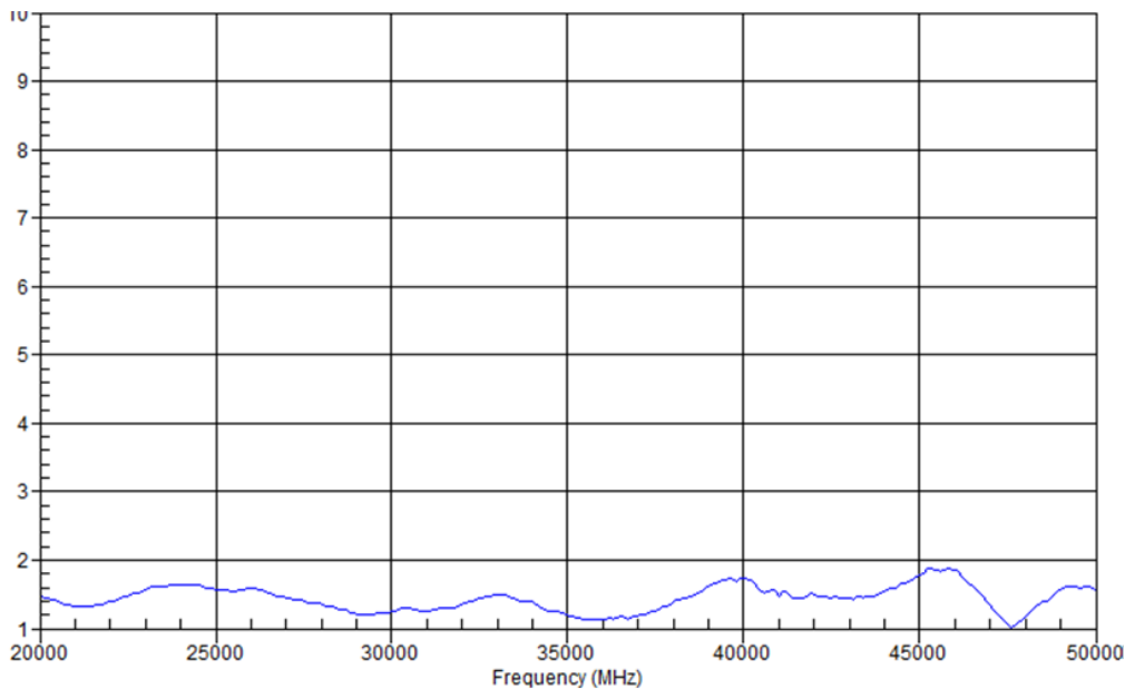
Figure 3: ERZ-HPA-2400-5000-28 Input VSWR
