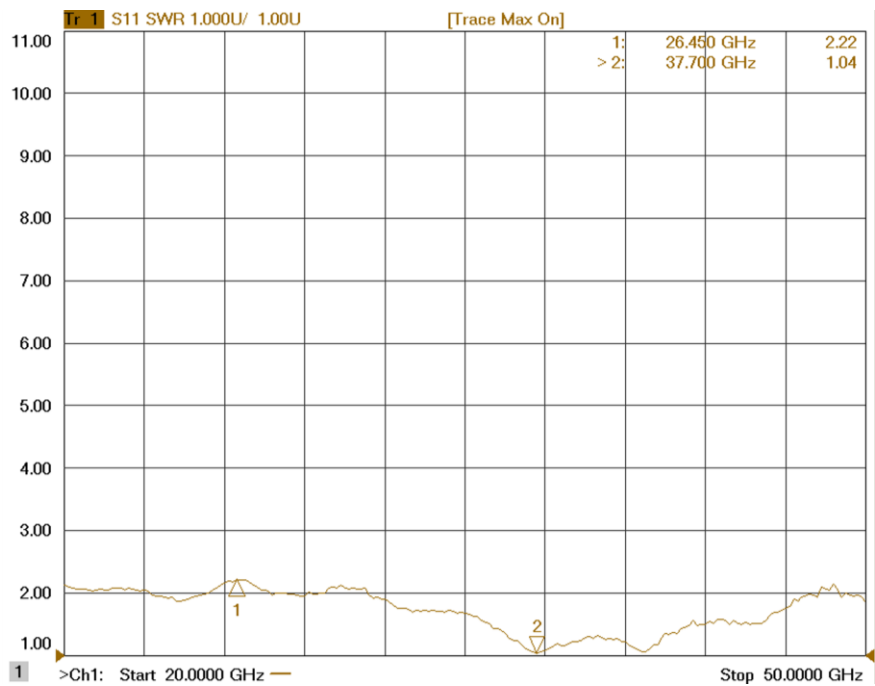
Figure 4: ERZ-HPA-2400-5000-28 Output VSWR
