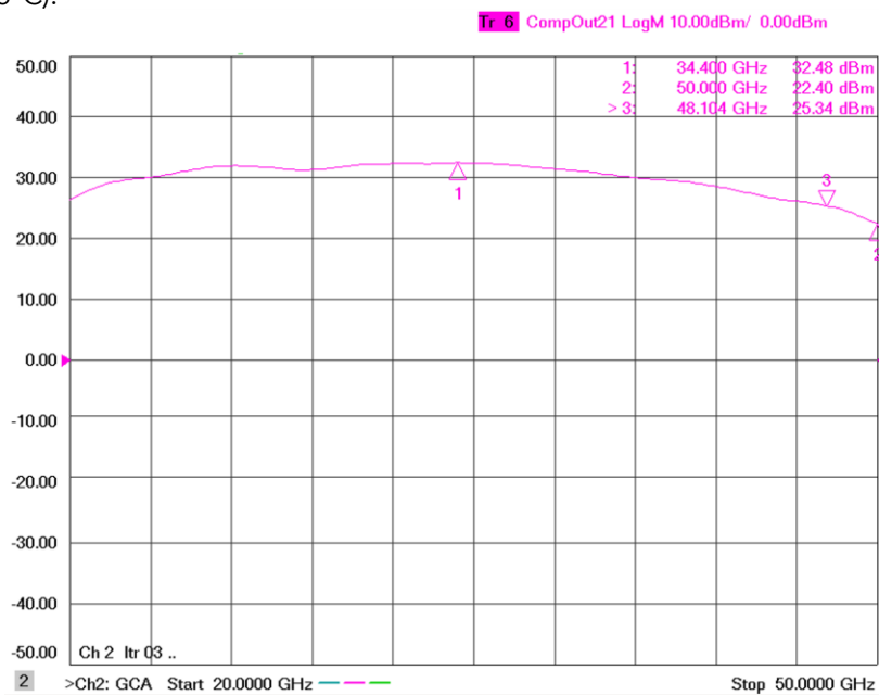
Figure 1: ERZ-HPA-2400-5000-28 Psat
