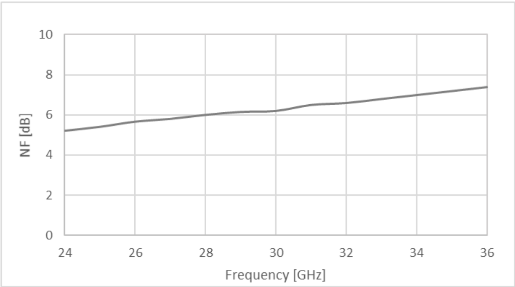
Figure 3: ERZ-HPA-2400-3600-27 Noise Figure
