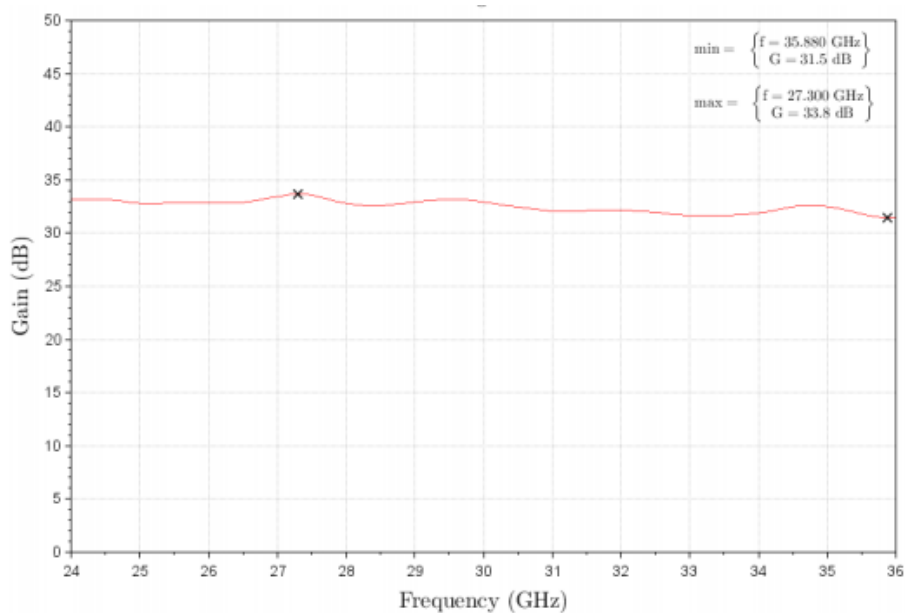
Figure 2: ERZ-HPA-2400-3600-27 Small Signal Gain
