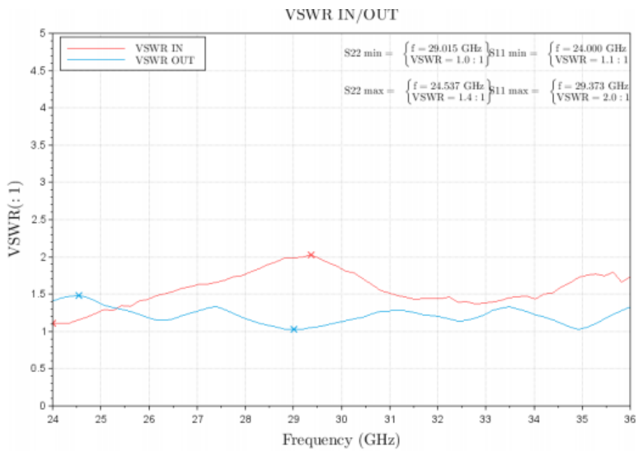
Figure 4: ERZ-HPA-2400-3600-27 Input&Output Matching
