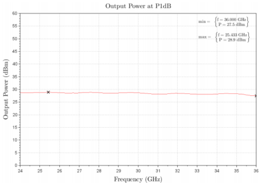
Figure 1: ERZ-HPA-2400-3600-27 P1dB
