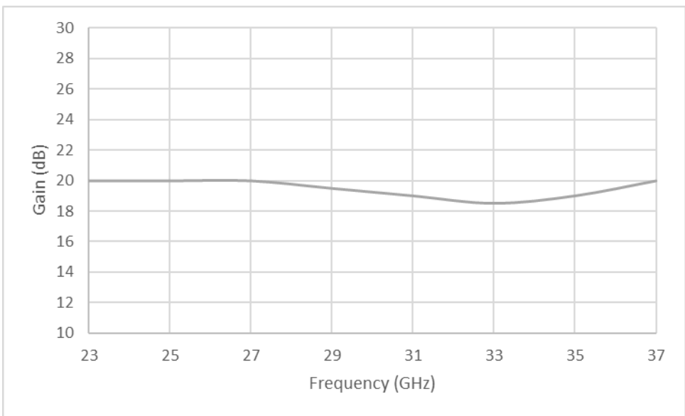
Figure 2: ERZ-HPA-2300-3700-25 Small Signal Gain
