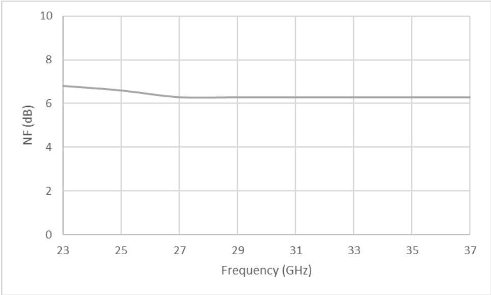
Figure 3: ERZ-HPA-2300-3700-25 Noise Figure
