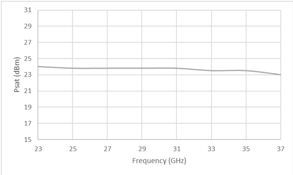
Figure 1: ERZ-HPA-2300-3700-25 P_{sat}
