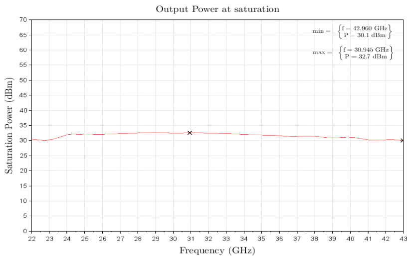
Figure 1: ERZ-HPA-2200-4300-32 Psat
