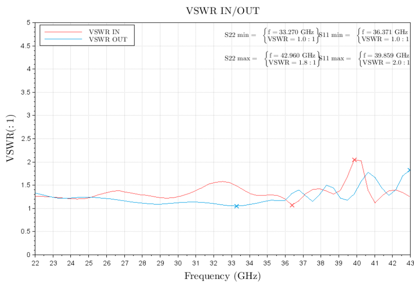
Figure 4: ERZ-HPA-2200-4300-32 Input&Output Matching
