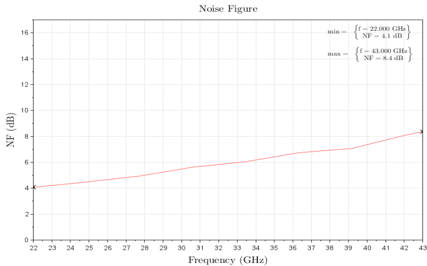
Figure 3: ERZ-HPA-2200-4300-32 NF
