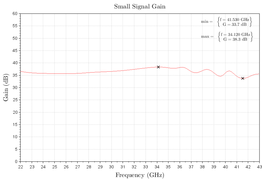
Figure 2: ERZ-HPA-2200-4300-32 Small Signal Gain
