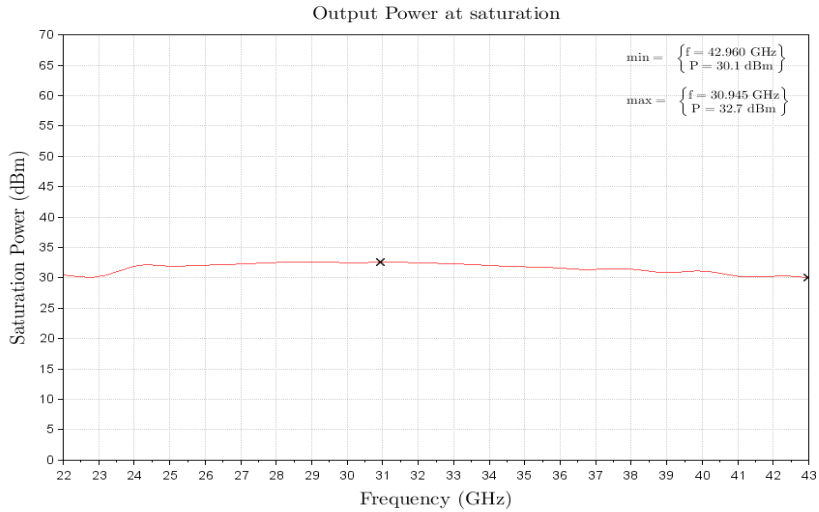
Figure 1: ERZ-HPA-2200-4300-32 Psat
