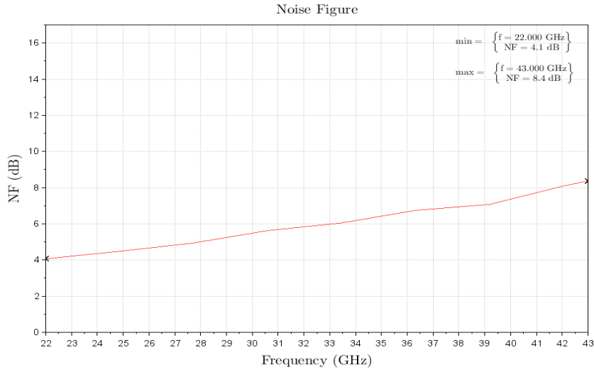
Figure 3: ERZ-HPA-2200-4300-32 NF
