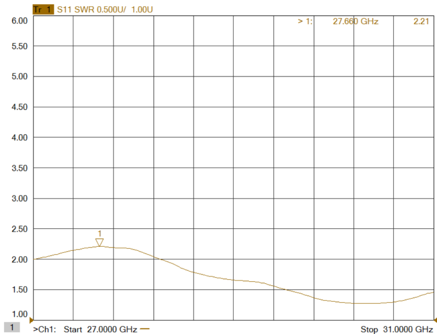
Figure 3: ERZ-HPA-1730-2120-44 Input Matching
