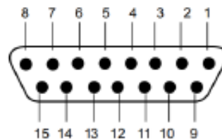
Figure 3-1: M83513/02-BN (female).
