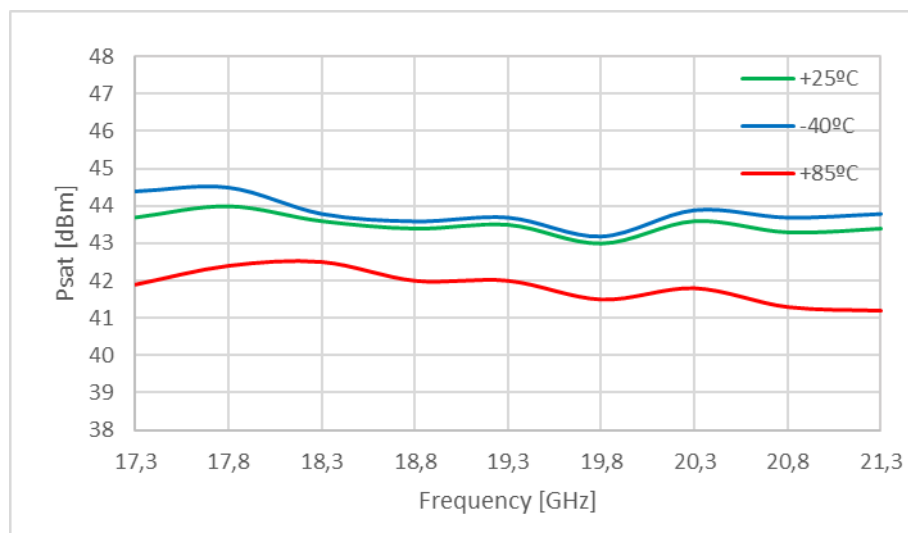
Figure 1: ERZ-HPA-1730-2120-44-NS Psat
