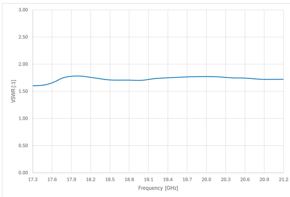
Figure 3: ERZ-HPA-1730-2120-44-NS Input Matching
