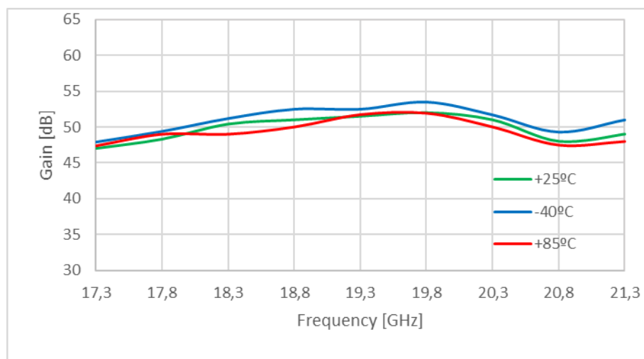
Figure 2: ERZ-HPA-1730-2120-44-NS Small Signal Gain
