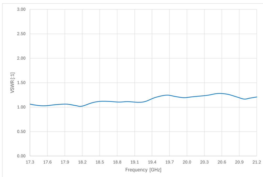
Figure 4: ERZ-HPA-1730-2120-44-NS Output Matching
