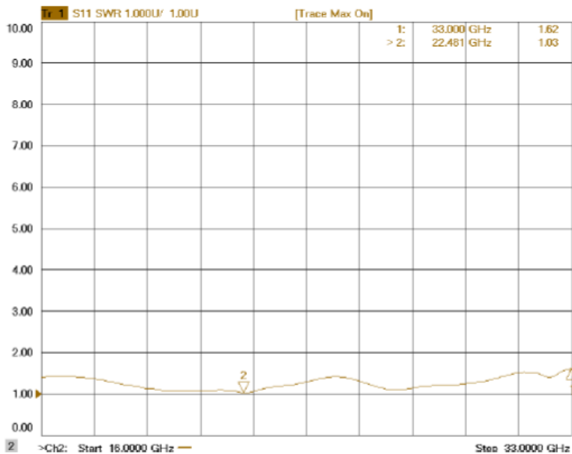
Figure 3: ERZ-HPA-1600-3300-24-E Input Matching
