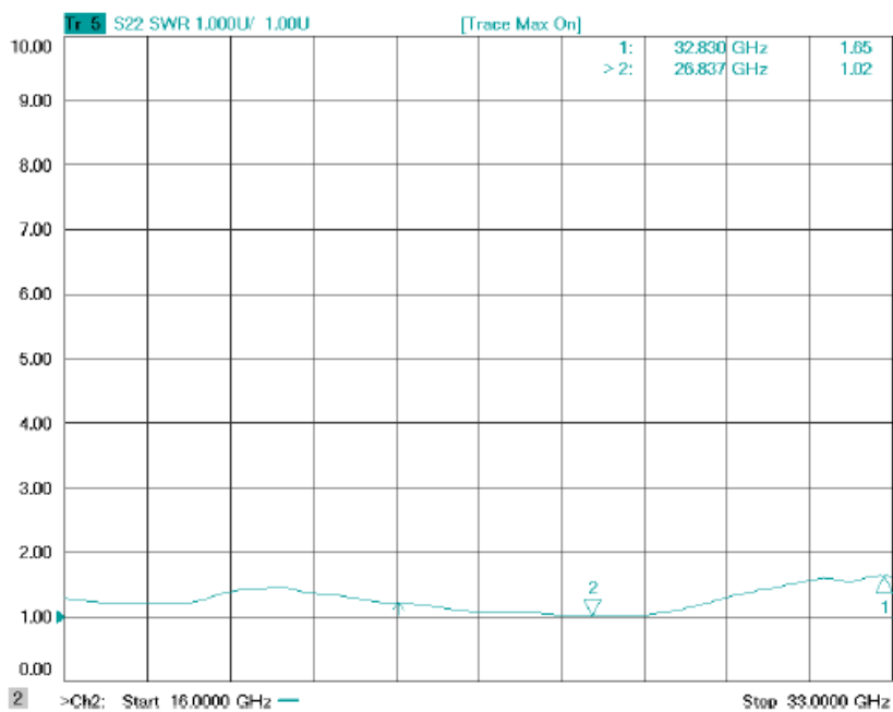
Figure 4: ERZ-HPA-1600-3300-24-E Output Matching
