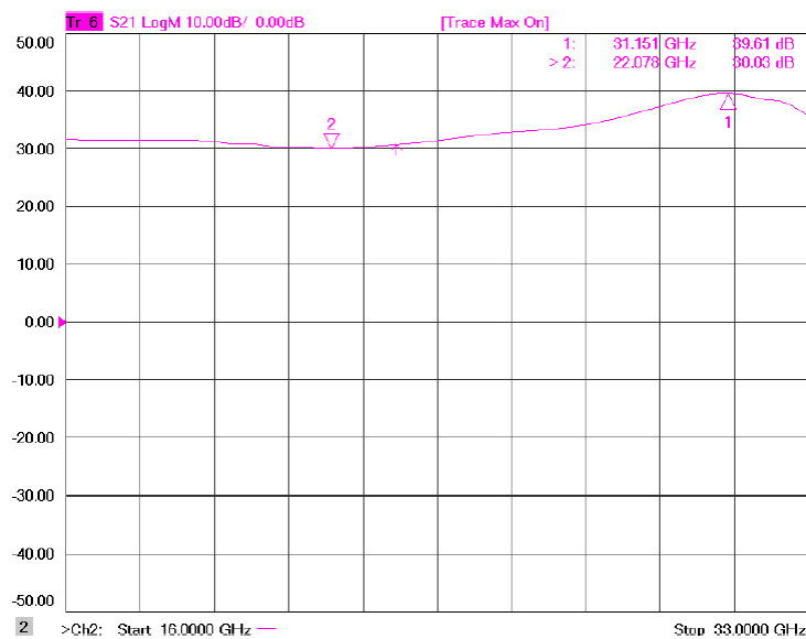
Figure 2: ERZ-HPA-1600-3300-24-E Small Signal Gain
