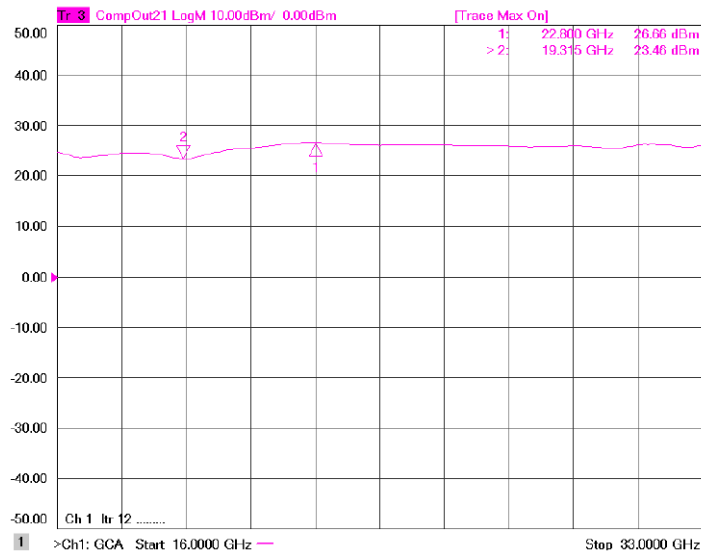
Figure 1: ERZ-HPA-1600-3300-24-E Psat
