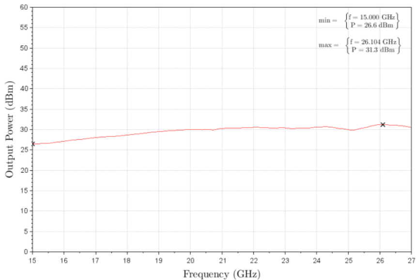
Figure 1: ERZ-HPA-1500-2700-29 P1dB
