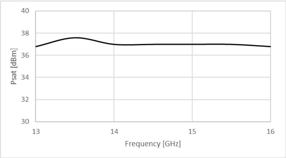
Figure 1: ERZ-HPA-1300-1600-37 Psat
