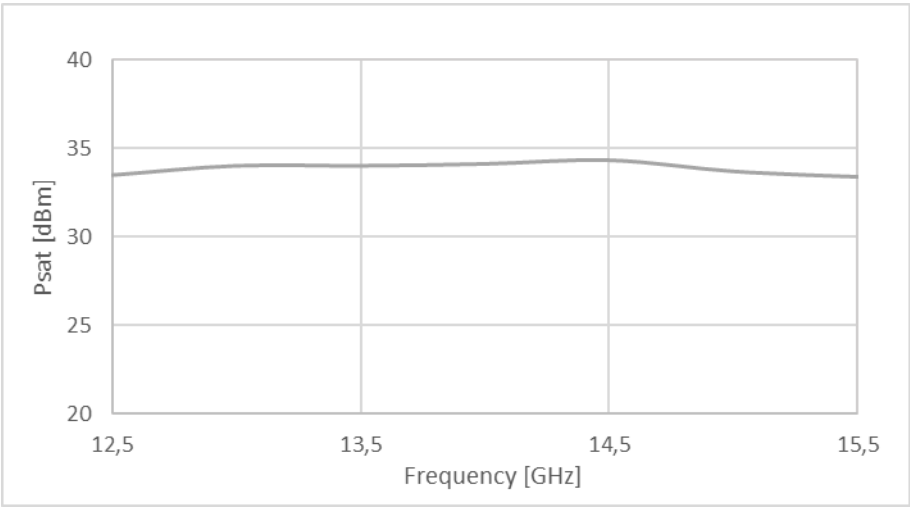
Figure 1: ERZ-HPA-1250-1550-34 Psat
