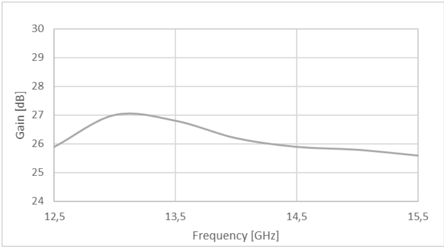
Figure 2: ERZ-HPA-1250-1550-34 Small Signal Gain
