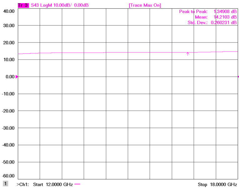
Figure 1-2: ERZ-HPA-1200-1800-27 Small Signal Gain
