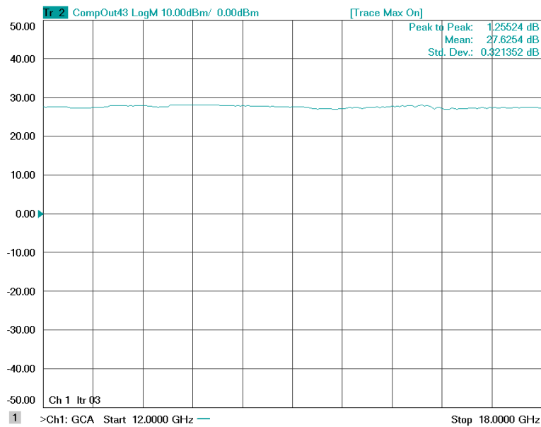
Figure 1-1: ERZ-HPA-1200-1800-27 P1dB
