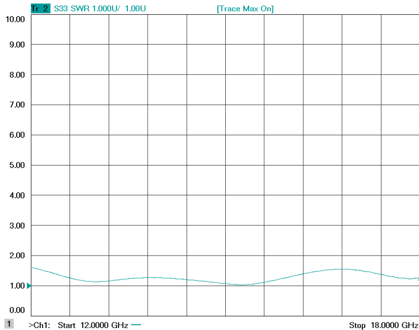
Figure 1-4: ERZ-HPA-1200-1800-27 Input Matching
