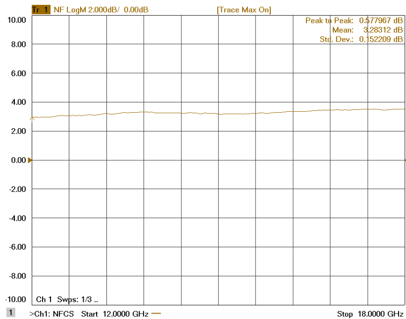
Figure 1-3: ERZ-HPA-1200-1800-27 Noise Figure
