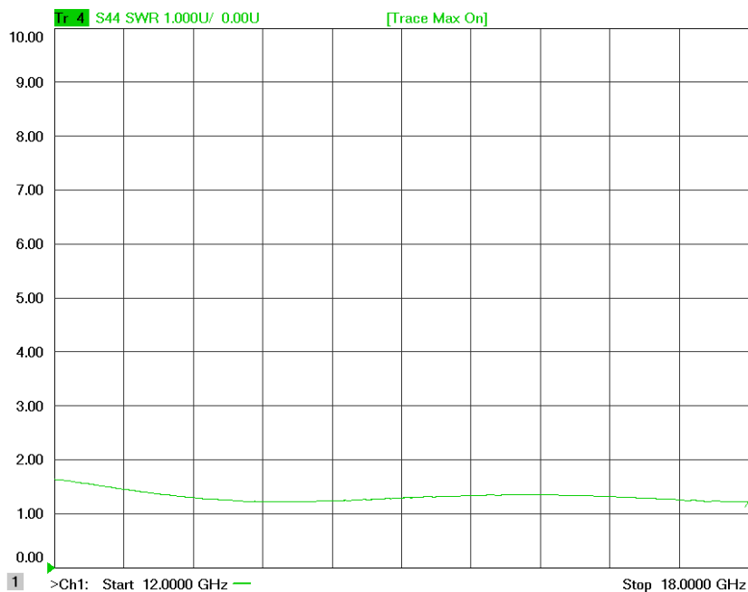
Figure 1-5: ERZ-HPA-1200-1800-27 Output Matching
