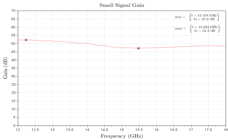
Figure 2: ERZ-HPA-1200-1800-27-E Small Signal Gain
