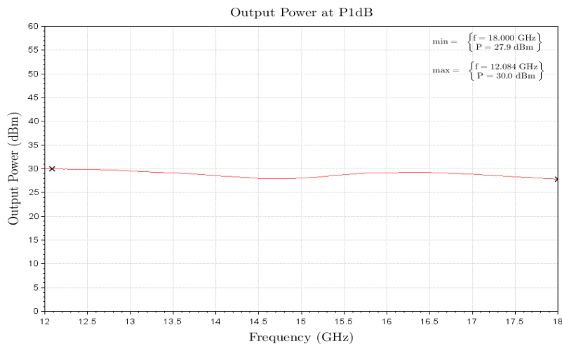
Figure 1: ERZ-HPA-1200-1800-27-E Output Power at P1dB
