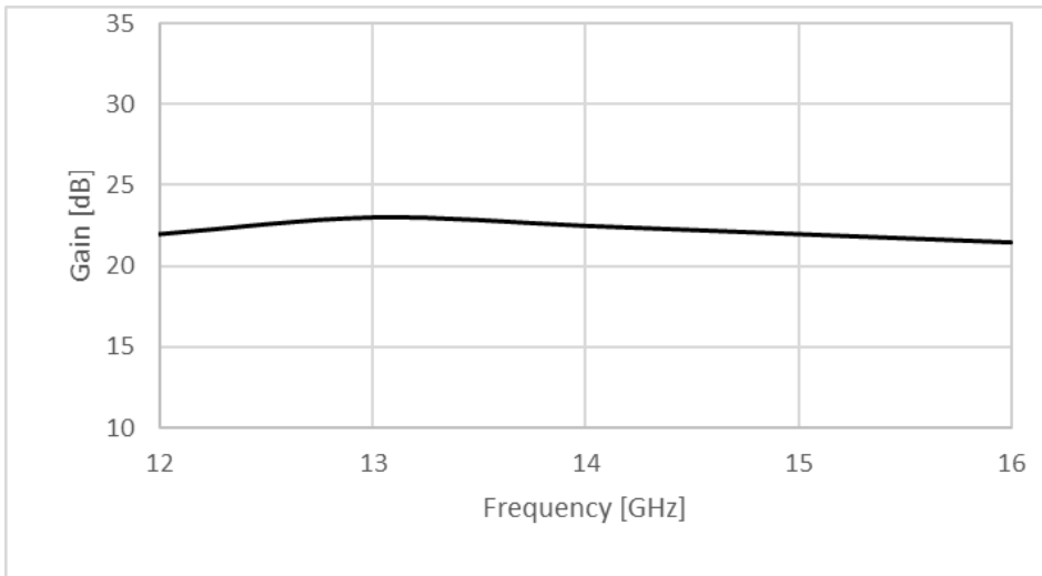
Figure 2: ERZ-HPA-1200-1600-26 Small Signal Gain
