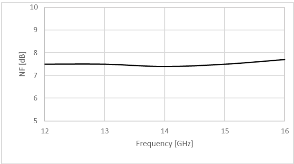
Figure 3: ERZ-HPA-1200-1600-26 Noise Figure
