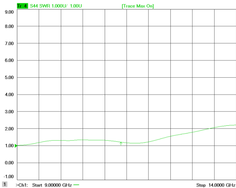
Figure 4: ERZ-HPA-0900-1400-34 Output Matching
