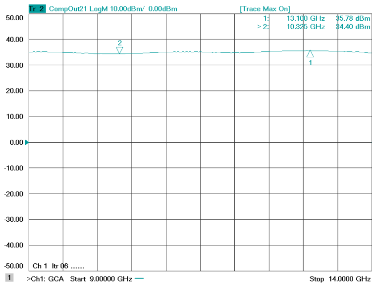
Figure 1: ERZ-HPA-0900-1400-34 Psat
