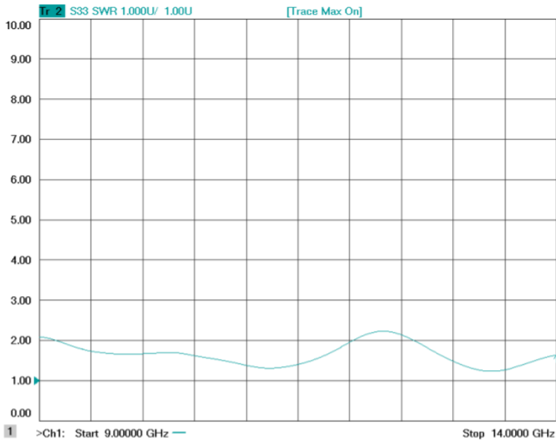
Figure 3: ERZ-HPA-0900-1400-34 Input Matching
