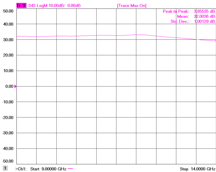
Figure 2: ERZ-HPA-0900-1400-34 Small Signal Gain
