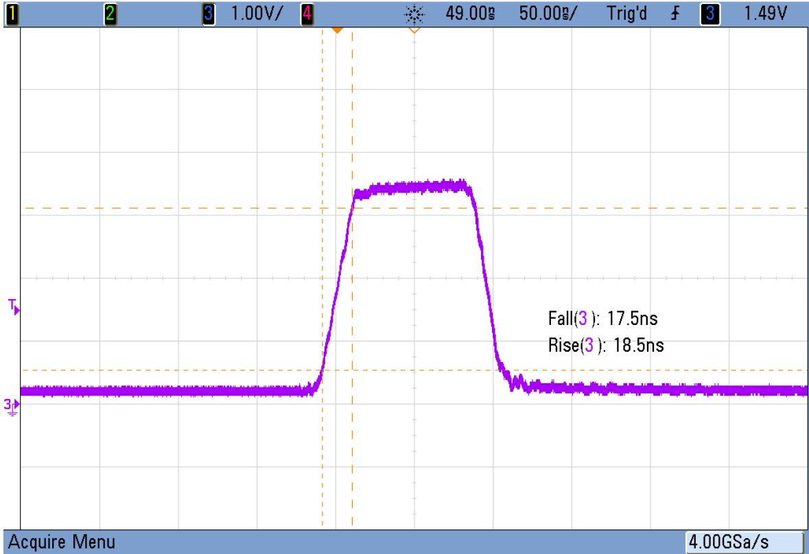
Figure 7: Detected Output Power Pulse at Psat
