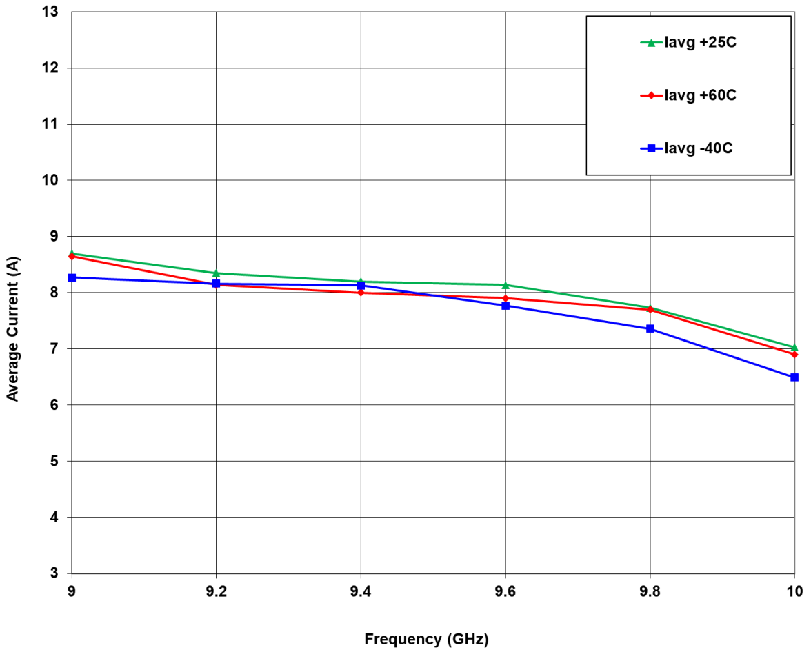
Figure 3: ERZ-HPA-0900-1000-56 Current (@28VDC) Vs Freq
