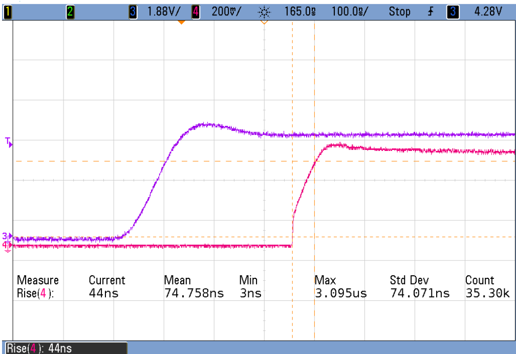
Figure 12: ERZ-HPA-0900-1000-56-M Switch ON time
