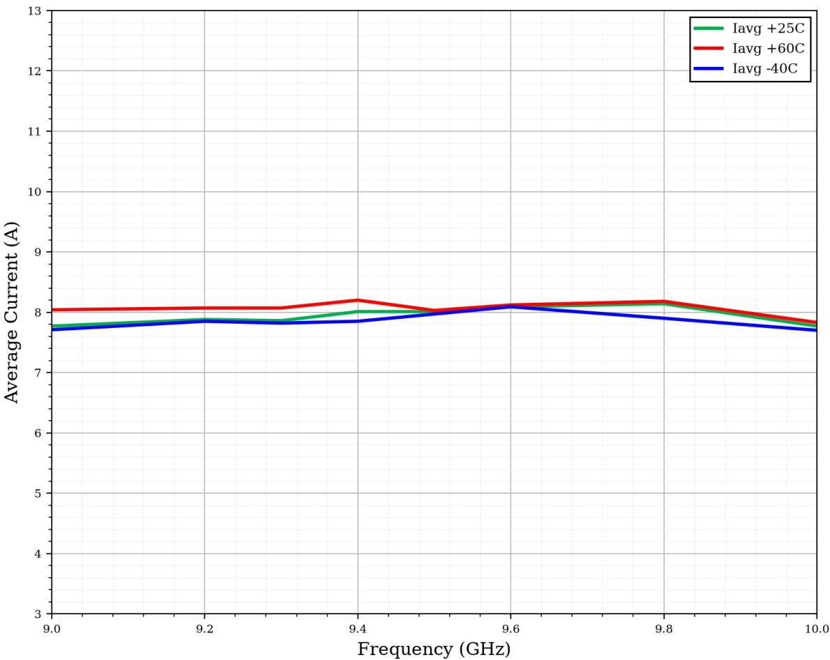
Figure 3: ERZ-HPA-0900-1000-56-M Current (@28VDC) Vs Freq
