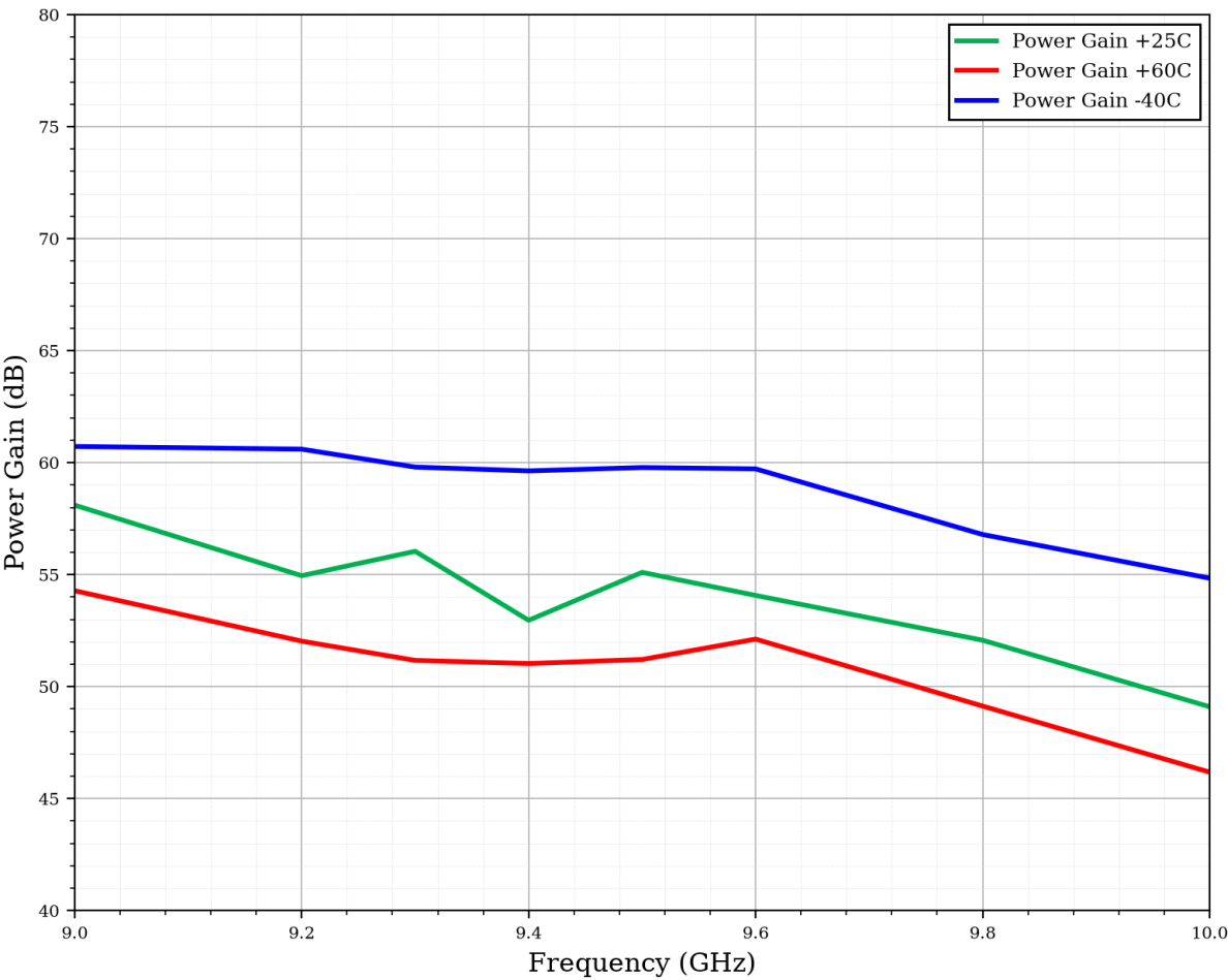
Figure 2: ERZ-HPA-0900-1000-56-M Power Gain Vs Freq
