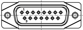
Figure 16: Control Connector. DSUB 15 Male Front View
