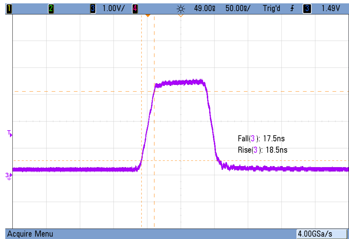
Figure 7: Detected Ouput Power Pulse at PSat
