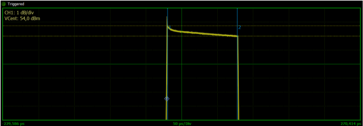
Figure 11: ERZ-HPA-0900-1000-56-M RF Output Pulse at 9.5 GHz
