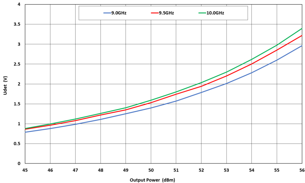
Figure 5: ERZ-HPA-0900-1000-56-M Pout detected Vs Pin
