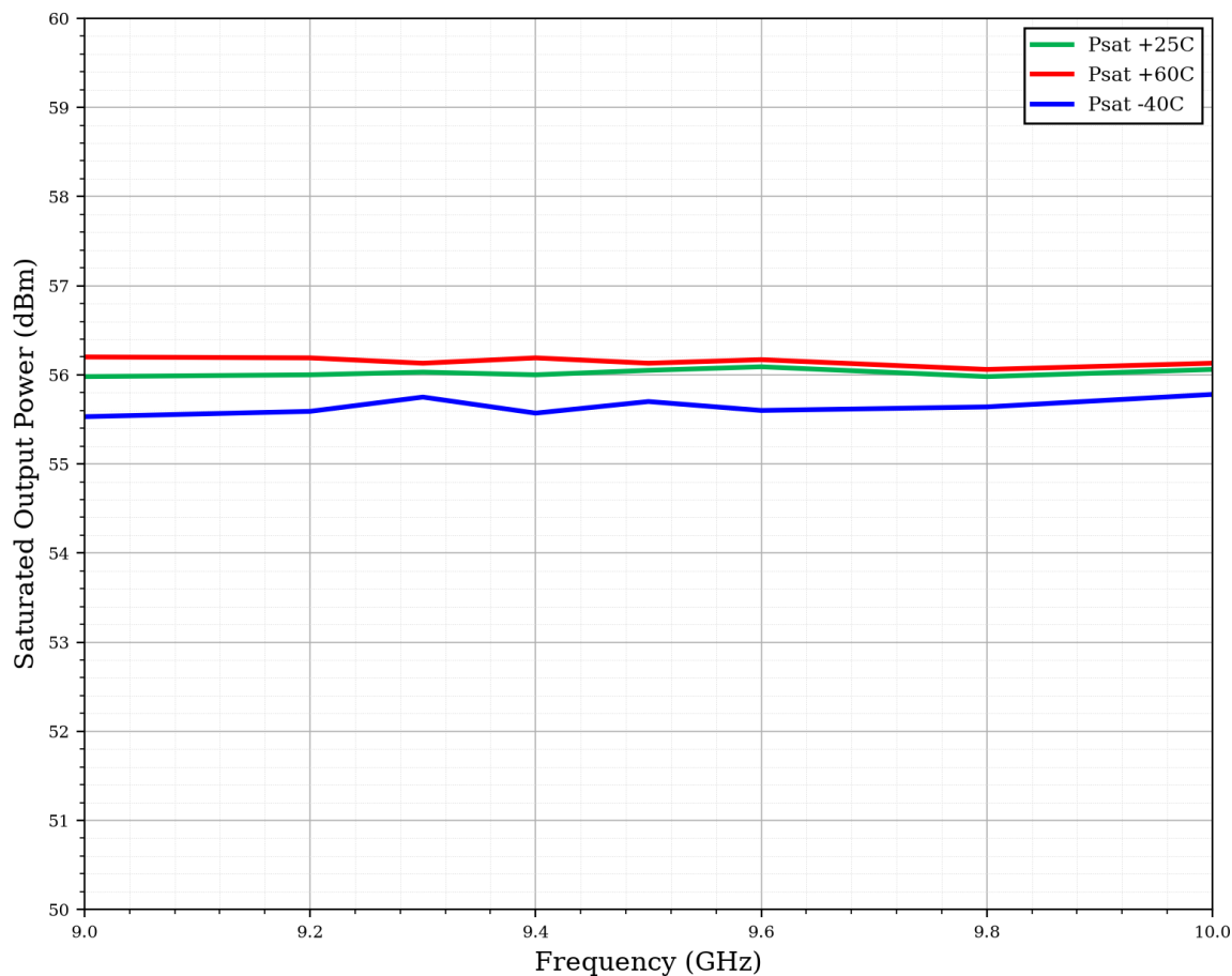
Figure 1: ERZ-HPA-0900-1000-56-M Psat Vs Freq
