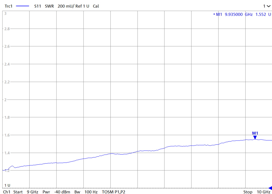
Figure 9: ERZ-HPA-0900-1000-56-M Input Matching Vs Frequency
