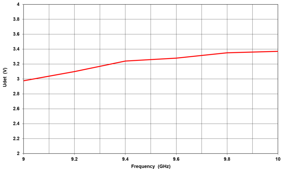
Figure 6: ERZ-HPA-0900-1000-56-M Pout detected at Pout 56 dBm
