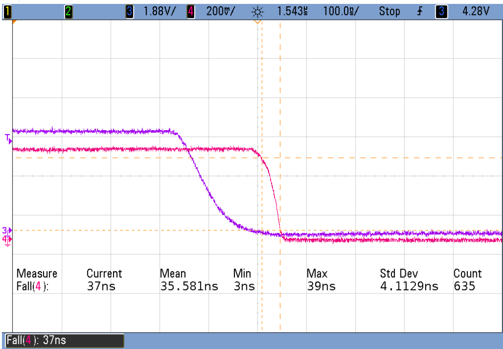
Figure 13: ERZ-HPA-0900-1000-56-M Switch OFF time
