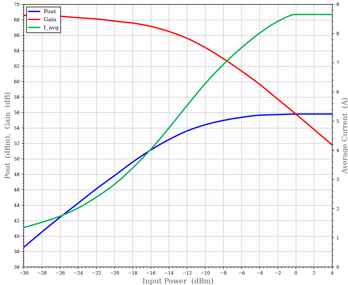
Figure 4: ERZ-HPA-0900-1000-56-M Pout, Gain and Power consumption Vs Pin
