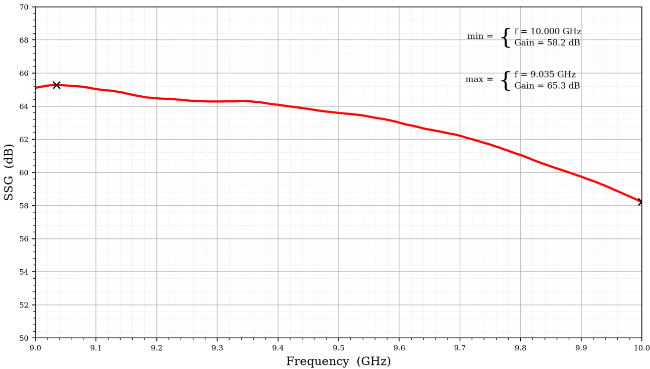
Figure 8: ERZ-HPA-0900-1000-56-M Small signal gain Vs Frequency
