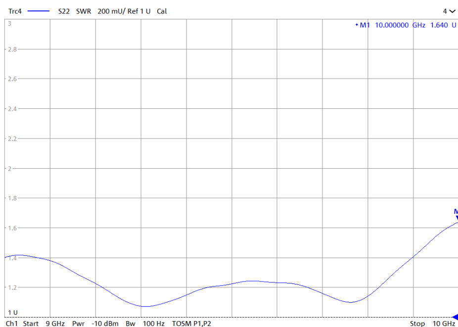
Figure 10: ERZ-HPA-0900-1000-56-M Output Matching Vs Frequency
