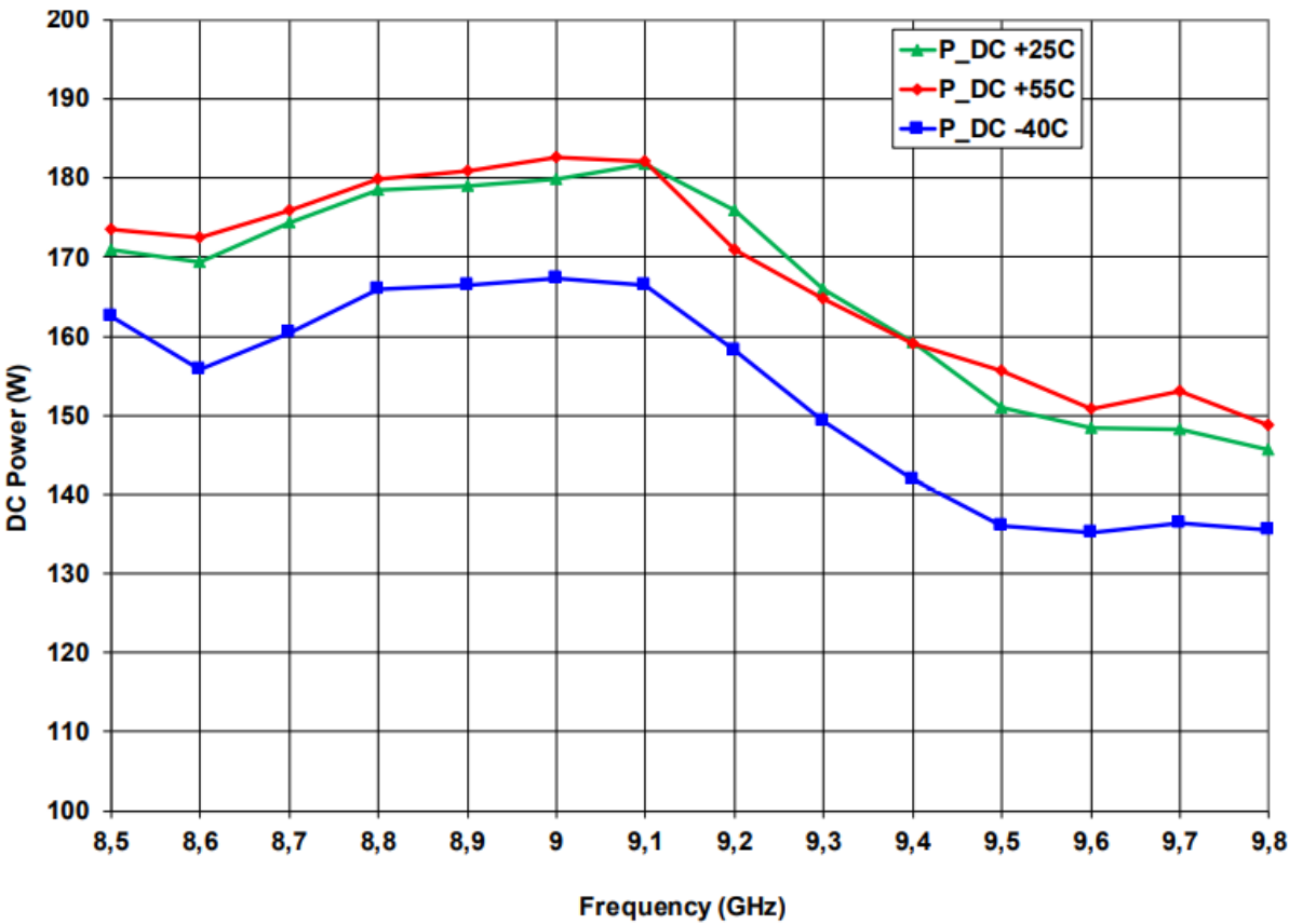
Figure 3: ERZ-HPA-0850-0980-55 Power Consumption Vs Freq
