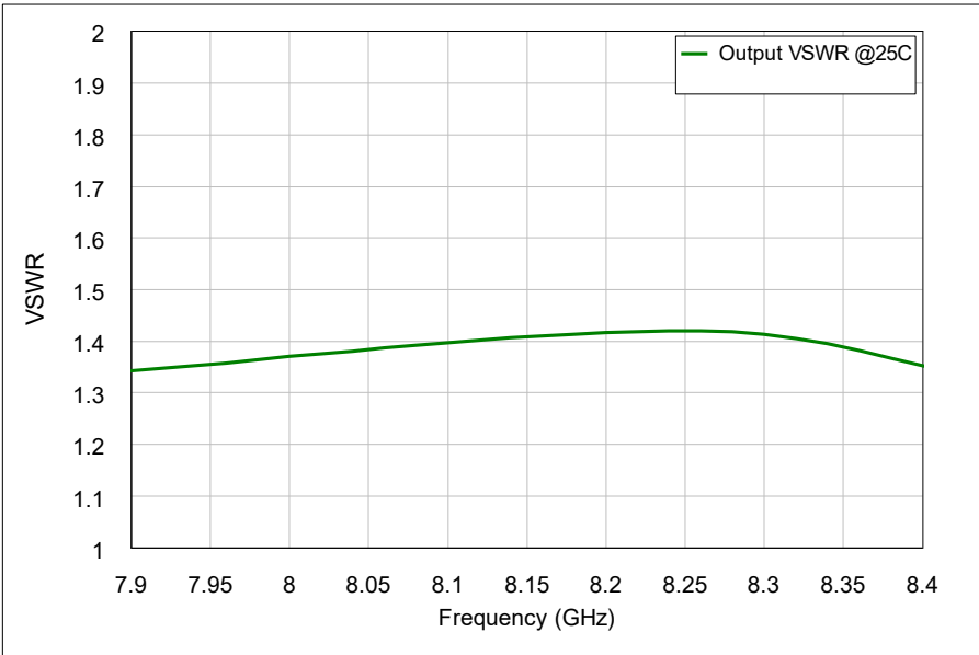
Figure 4: ERZ-HPA-0790-0840-46 Output Matching
