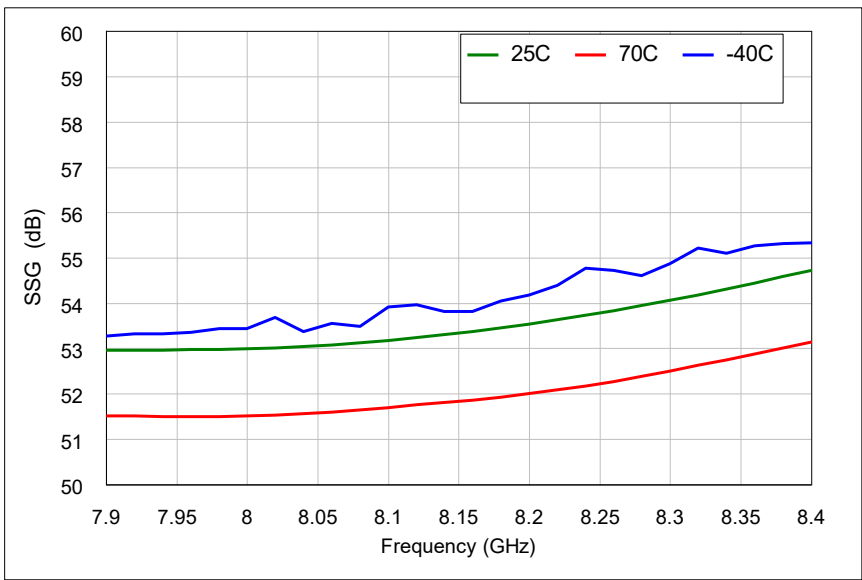
Figure 2: ERZ-HPA-0790-0840-46 Small Signal Gain
