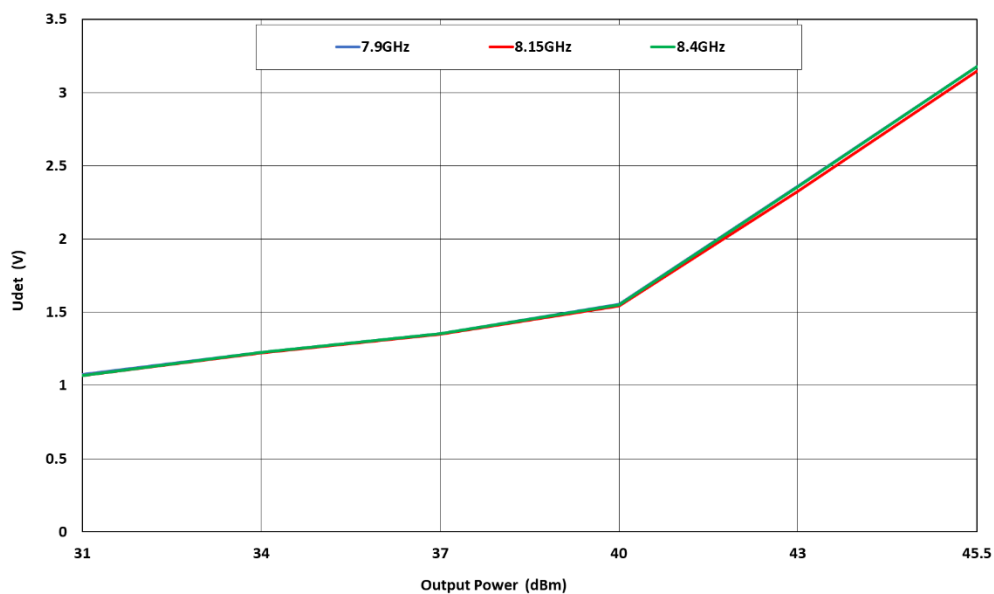
Figure 7: ERZ-HPA-0790-0840-46 Output power detector
