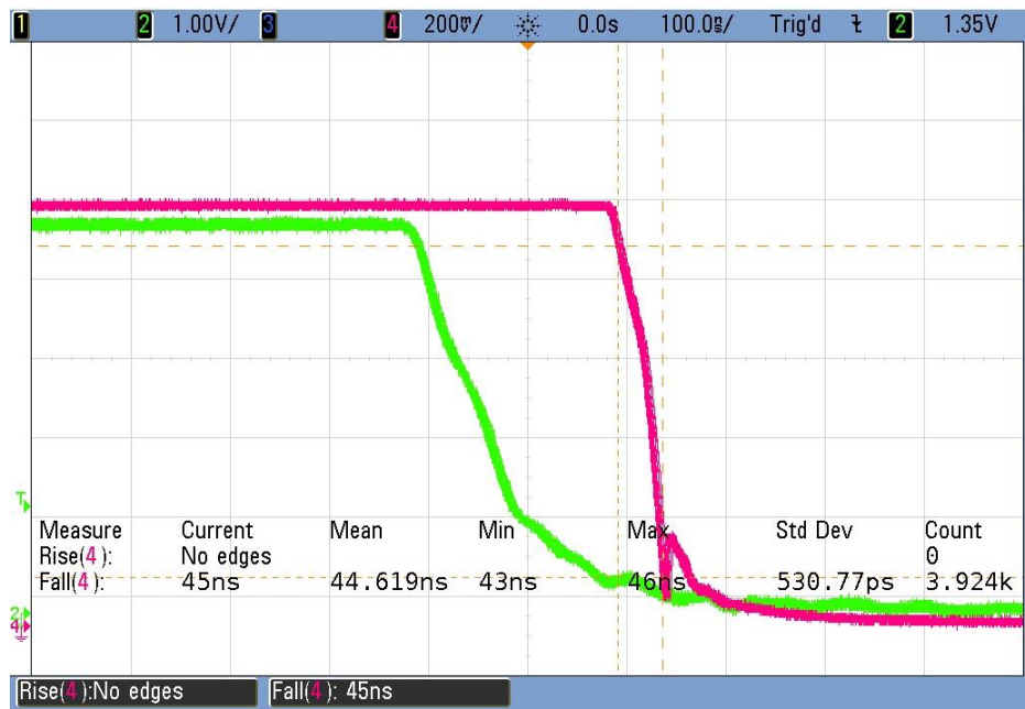
Figure 6: ERZ-HPA-0790-0840-46 Switch OFF Time
