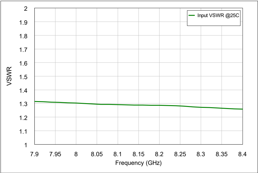
Figure 3: ERZ-HPA-0790-0840-46 Input Matching
