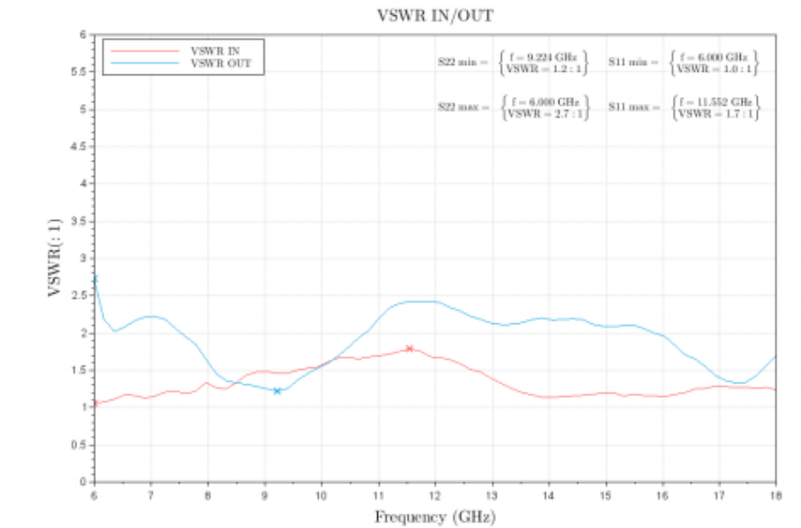
Figure 5: ERZ-HPA-0600-1800-40-E Input and Output Matching
