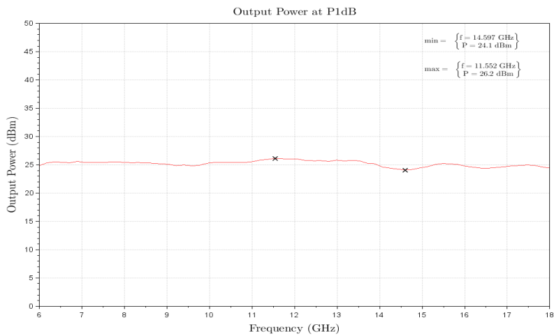
Figure 1: ERZ-HPA-0600-1800-24 Output Power at P1dB
