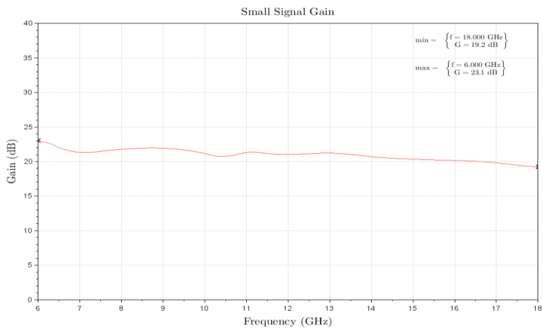
Figure 2: ERZ-HPA-0600-1800-24 Small Signal Gain
