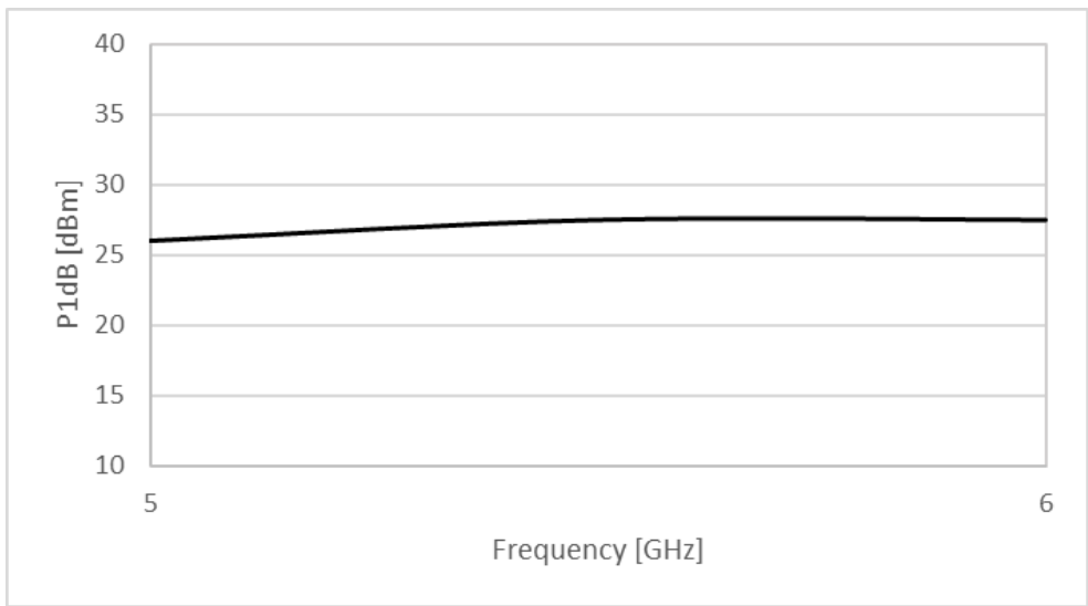
Figure 1: ERZ-HPA-0500-0600-25 P1dB
