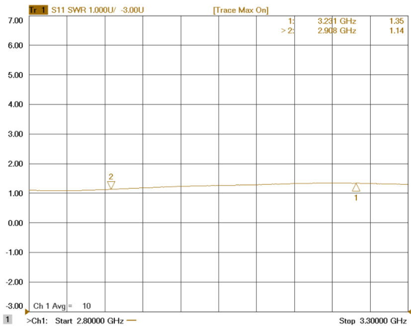
Figure 1-5: ERZ-HPA-0280-0330-40 Output Matching
