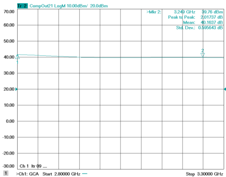
Figure 1-1: ERZ-HPA-0280-0330-40 P1dB
