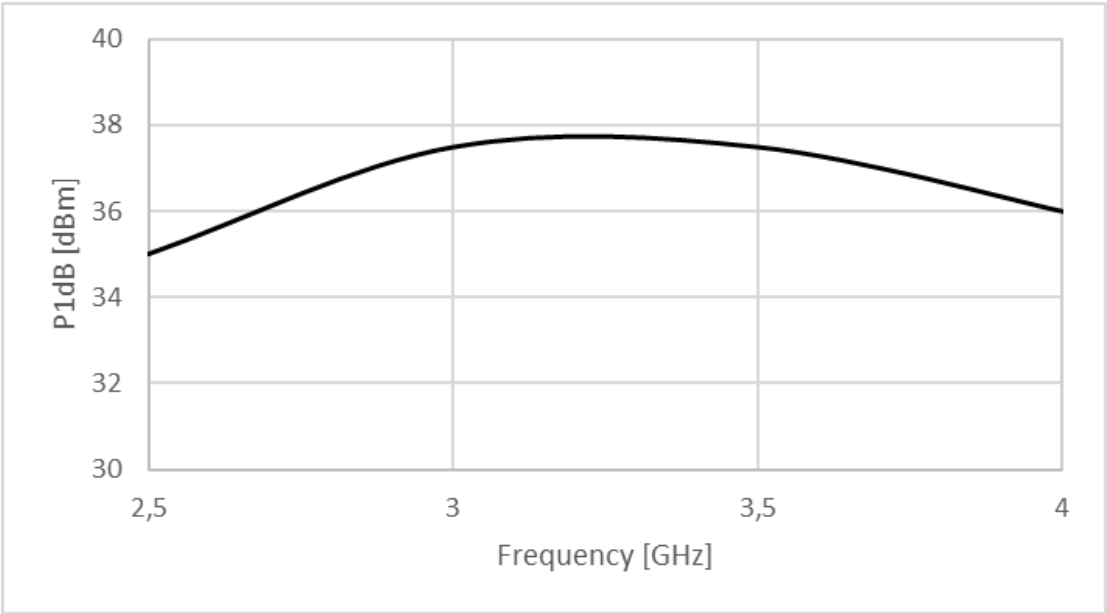
Figure 1: ERZ-HPA-0250-0400-35 P1dB
