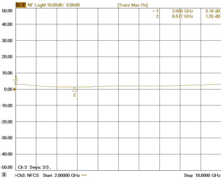
Figure 4: ERZ-HPA-0200-1800-30 Noise Figure
