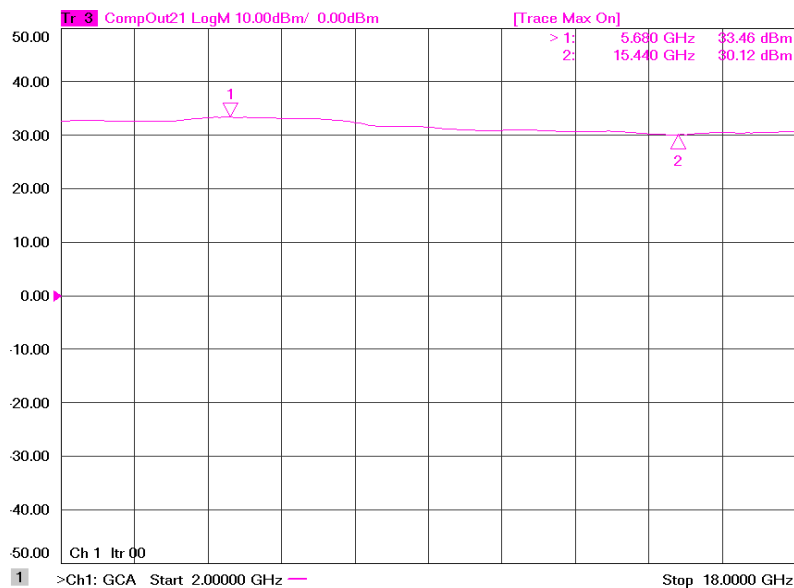
Figure 1: ERZ-HPA-0200-1800-30 P1dB
