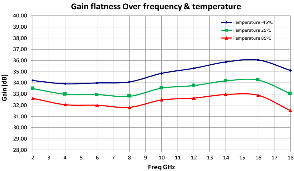
Figure 3: ERZ-HPA-0200-1800-30 Small Signal Gain Vs Temperature
