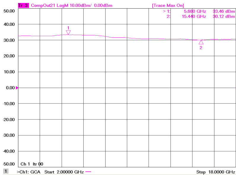
Figure 1: ERZ-HPA-0200-1800-30 P1dB
