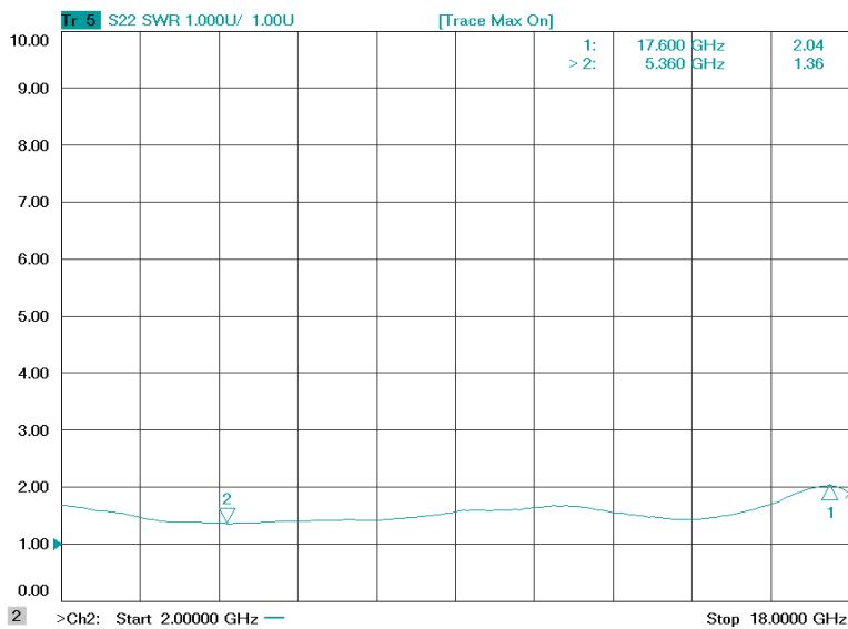
Figure 6: ERZ-HPA-0200-1800-30 Output Matching
