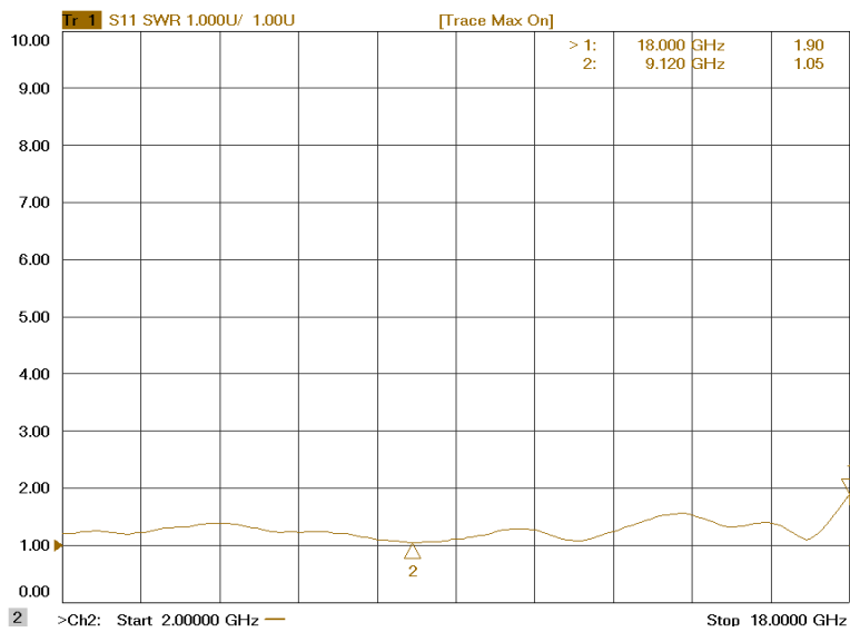
Figure 5: ERZ-HPA-0200-1800-30 Input Matching
