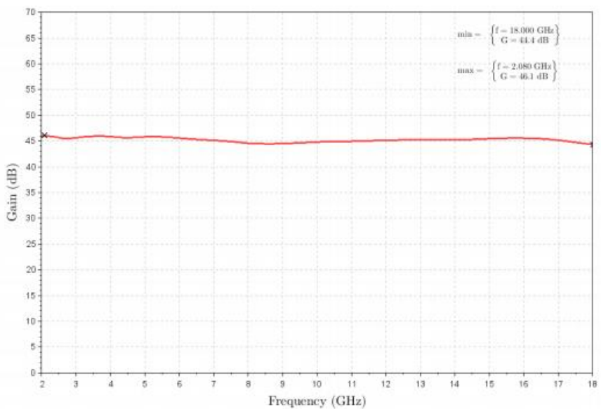
Figure 2: ERZ-HPA-0200-1800-30-E Small Signal Gain
