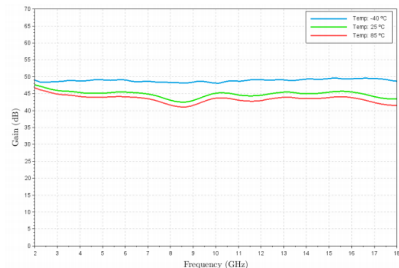
Figure 3: ERZ-HPA-0200-1800-30-E Small Signal Gain Vs Temperature
