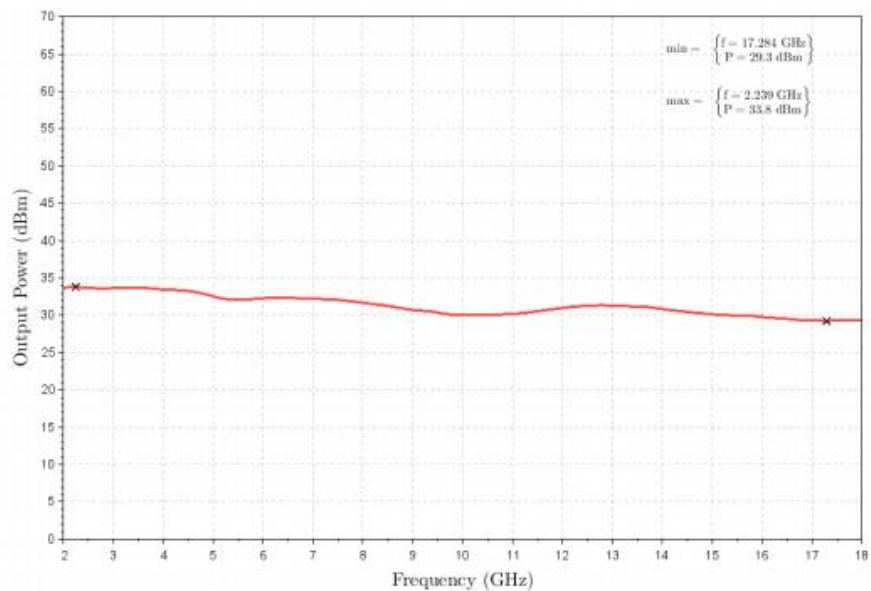
Figure 1: ERZ-HPA-0200-1800-30-E P1dB
