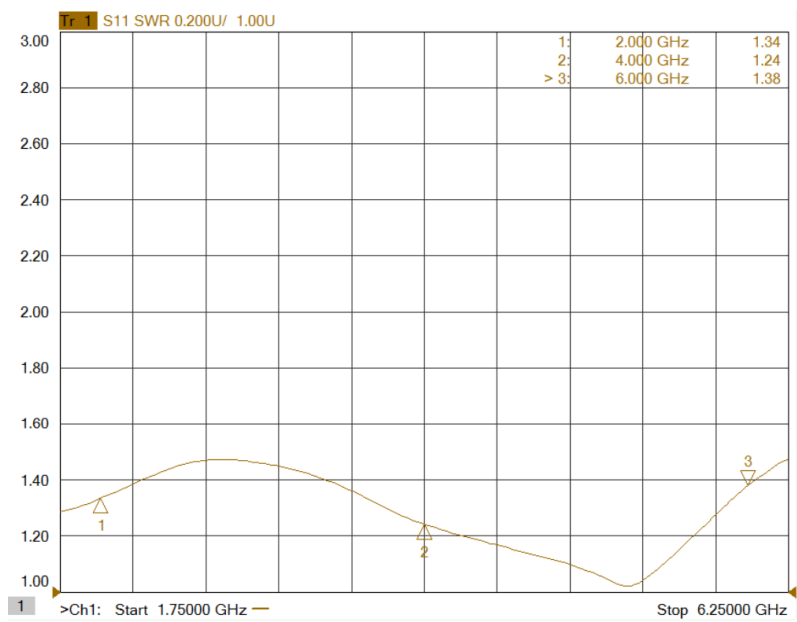
Figure 7: ERZ-HPA-0200-0400-43 Input Matching
