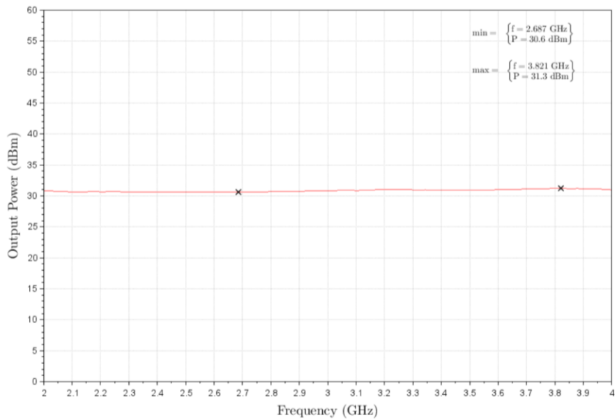
Figure 1: ERZ-HPA-0200-0400-30 P1dB
