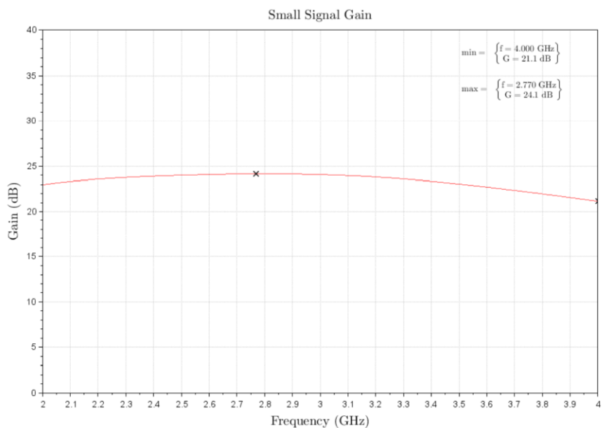
Figure 2: ERZ-HPA-0200-0400-24 Small Signal Gain
