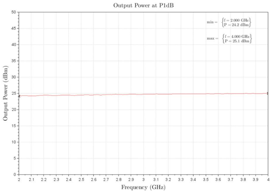
Figure 1: ERZ-HPA-0200-0400-24 P1dB
