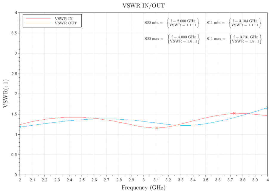
Figure 3: ERZ-HPA-0200-0400-24 Input & Output Matching
