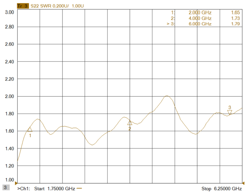
Figure 8: ERZ-HPA-0175-0625-43 Output Matching
