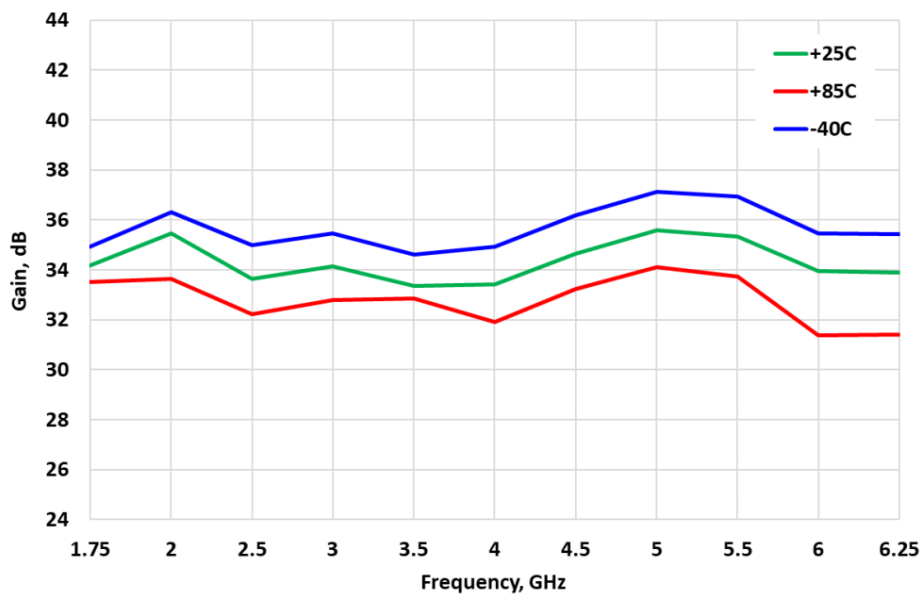
Figure 3: ERZ-HPA-0175-0625-43 PowerGain
