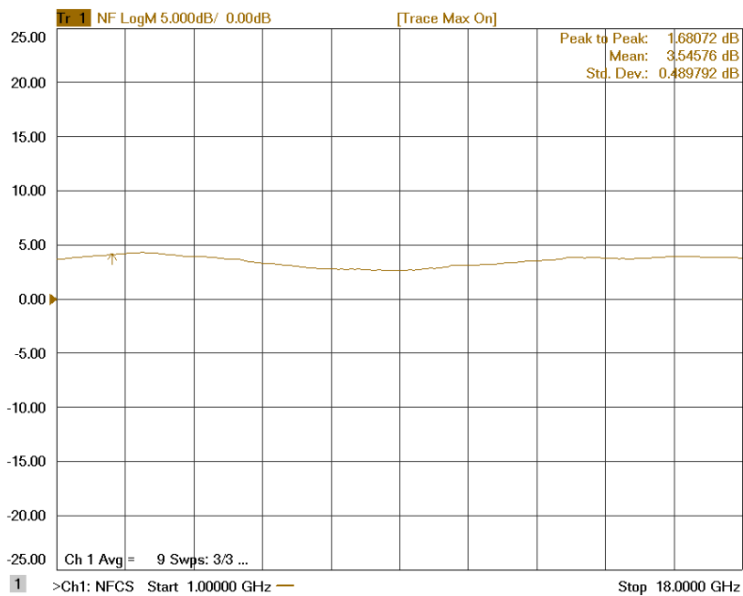
Figure 3: ERZ-HPA-0100-1800-21 Noise Figure
