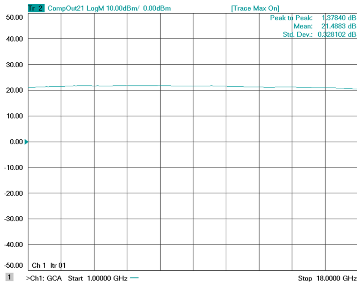
Figure 1: ERZ-HPA-0100-1800-21 P1dB
