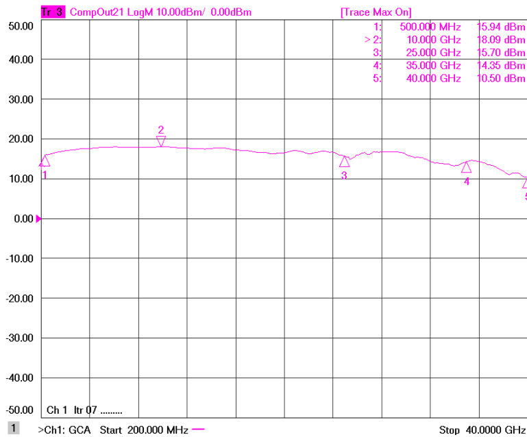
Figure 1: ERZ-HPA-0050-4000-8 P1dB
