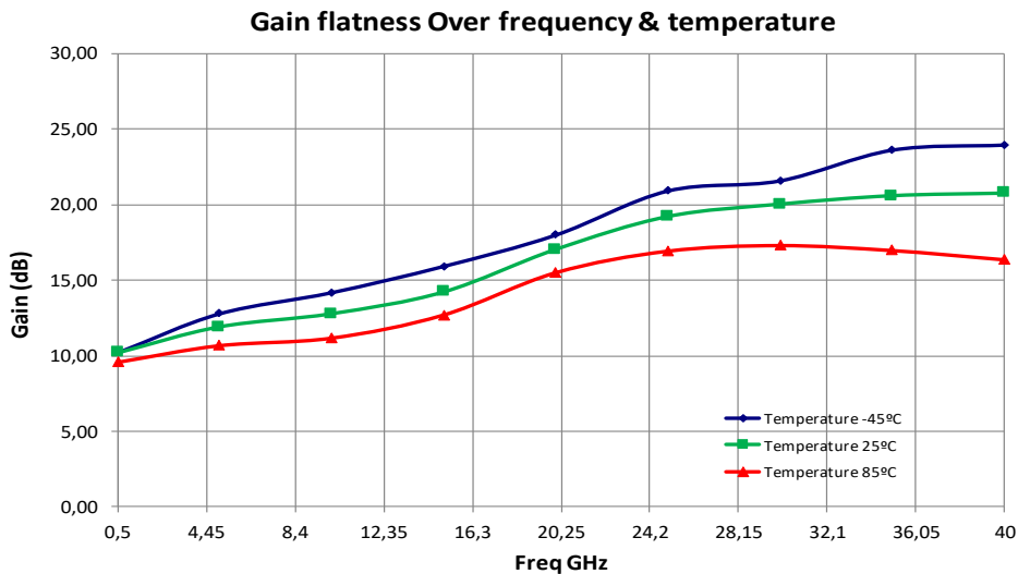
Figure 3: ERZ-HPA-0050-4000-8 Small Signal Gain Vs Temperature
