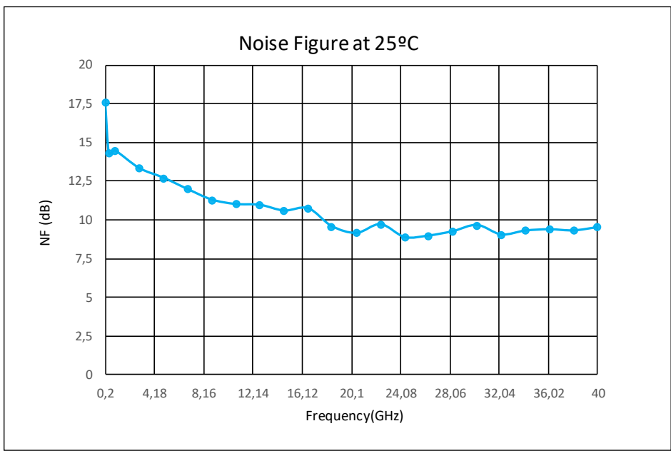
Figure 4: ERZ-HPA-0050-4000-8 NF
