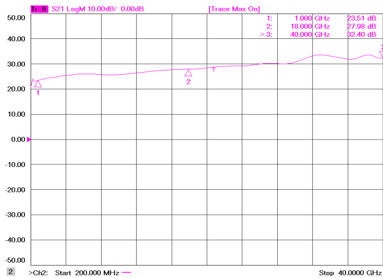
Figure 2: ERZ-HPA-0050-4000-12 Small Signal Gain
