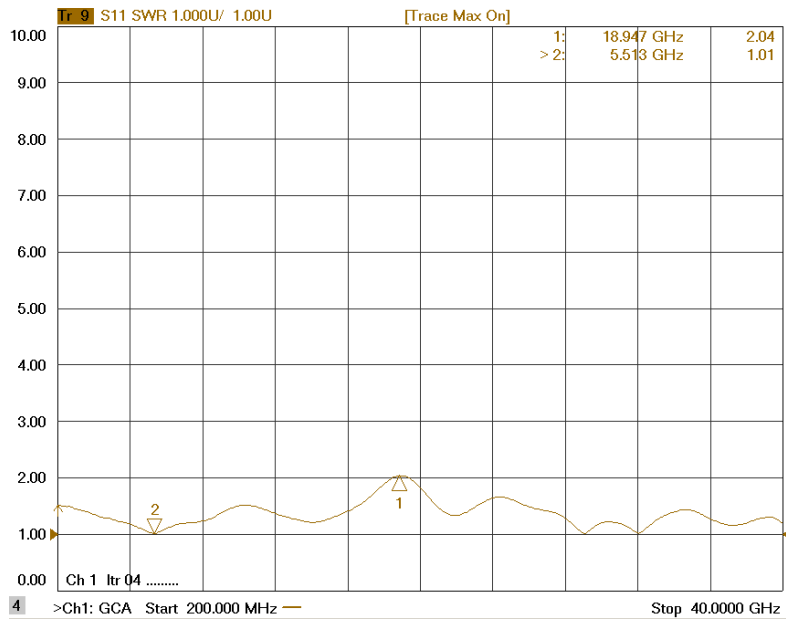
Figure 4: ERZ-HPA-0050-4000-12 Input Matching
