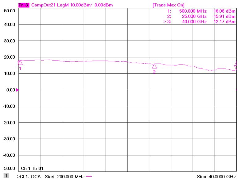
Figure 1: ERZ-HPA-0050-4000-12 P1dB
