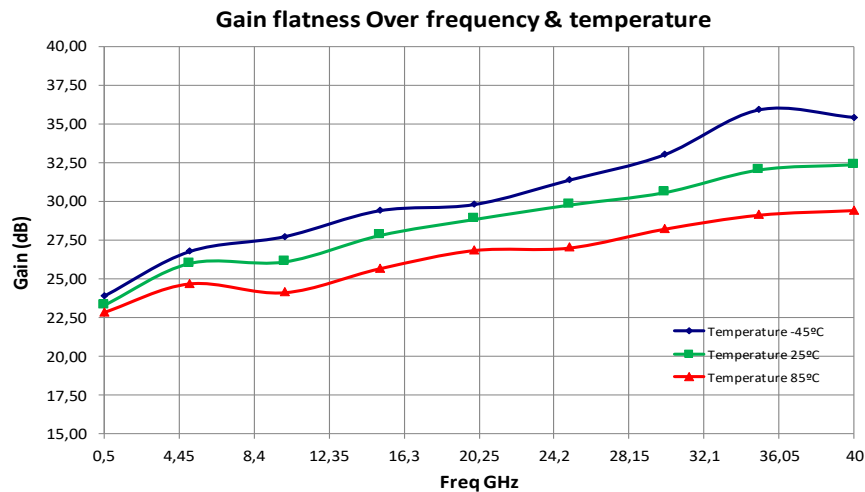
Figure 3: ERZ-HPA-0050-4000-12 Small Signal Gain Vs Temperature
