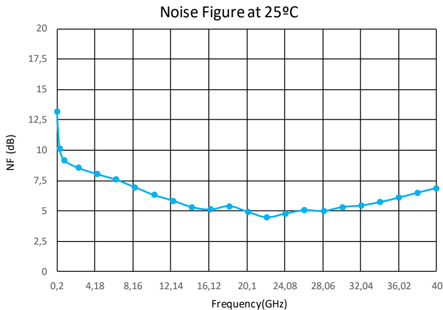
Figure 4: ERZ-HPA-0050-4000-12 NF
