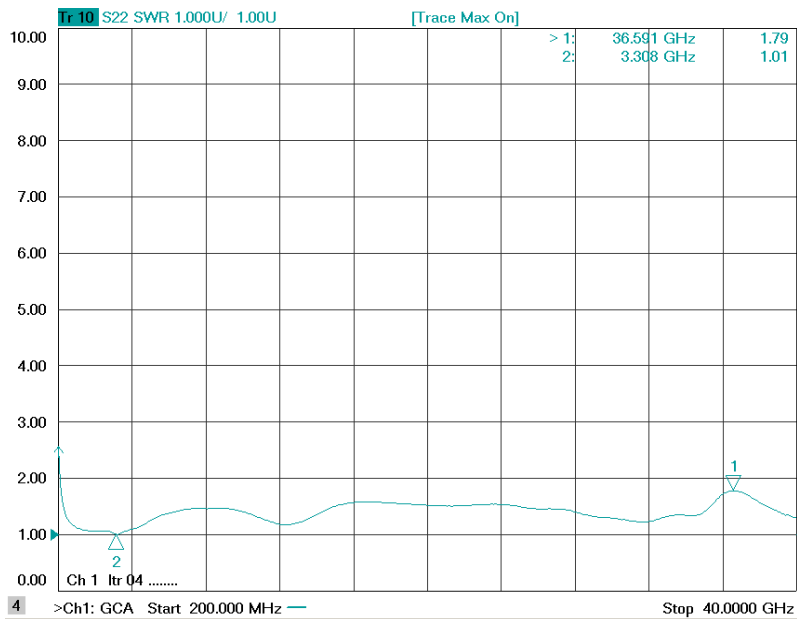
Figure 5: ERZ-HPA-0050-4000-12 Output Matching
