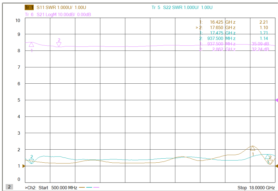
Figure 2: ERZ-HPA-0050-1800-30 S-parameters
