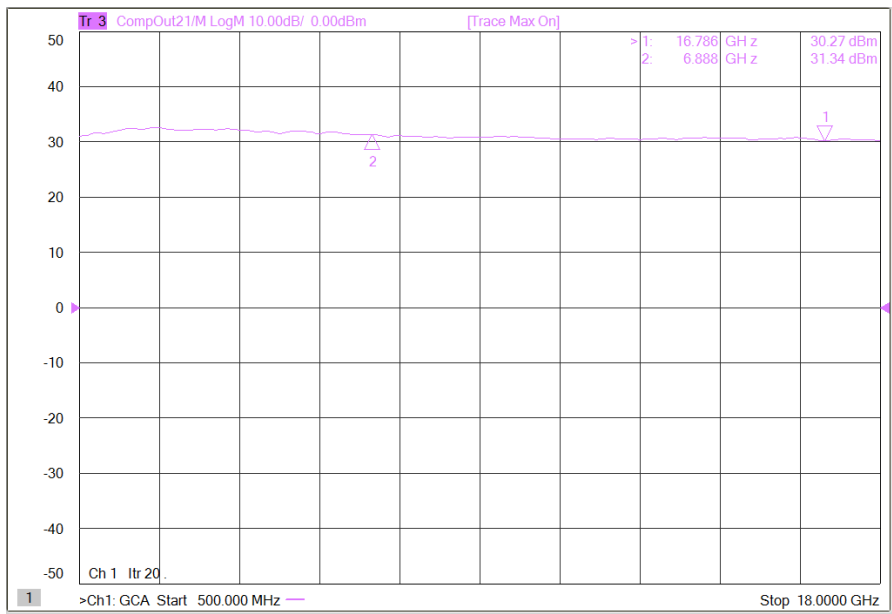
Figure 1: ERZ-HPA-0050-1800-30 P1dB
